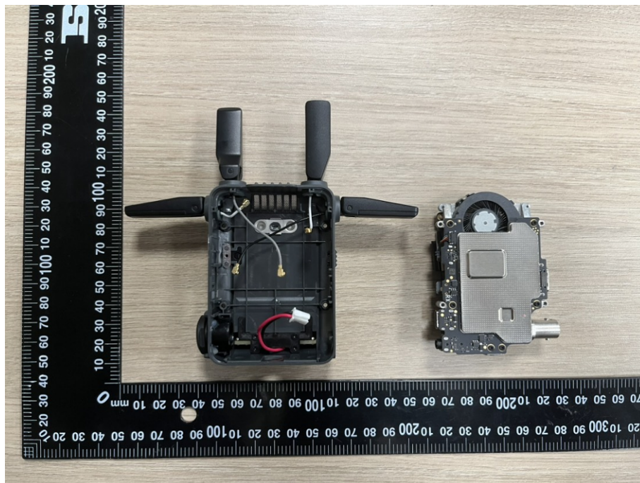
Fig.2. Internal view-02
