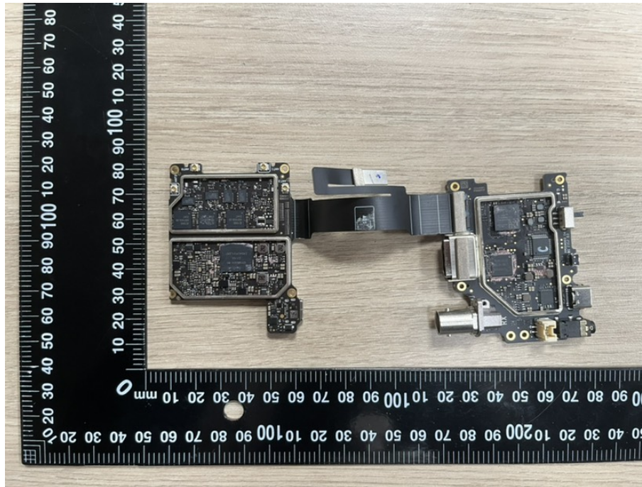
Fig.4. Mainboard view-01
