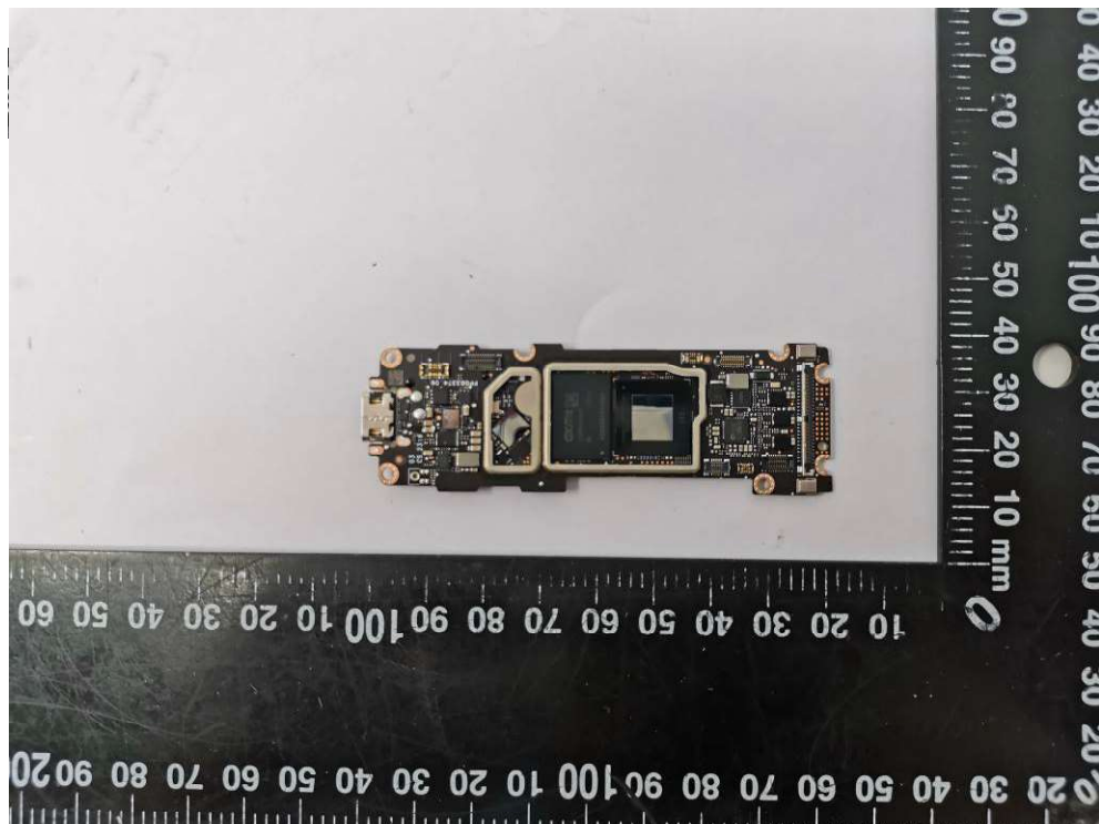
Fig.8 Mainboard view-01
