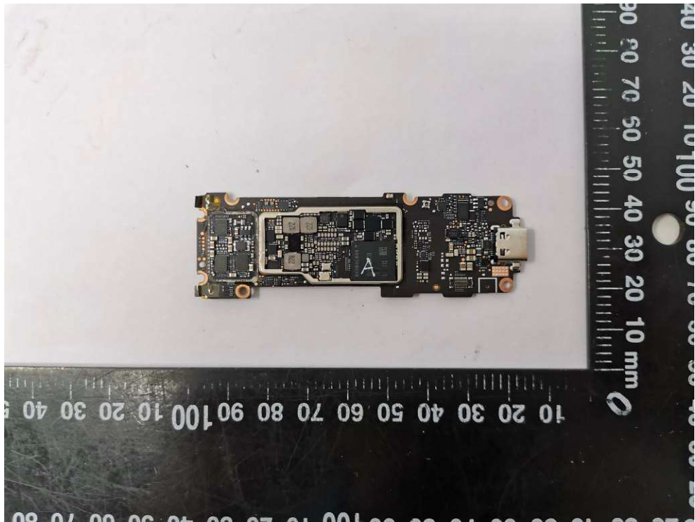
Fig.9 Mainboard view-02
