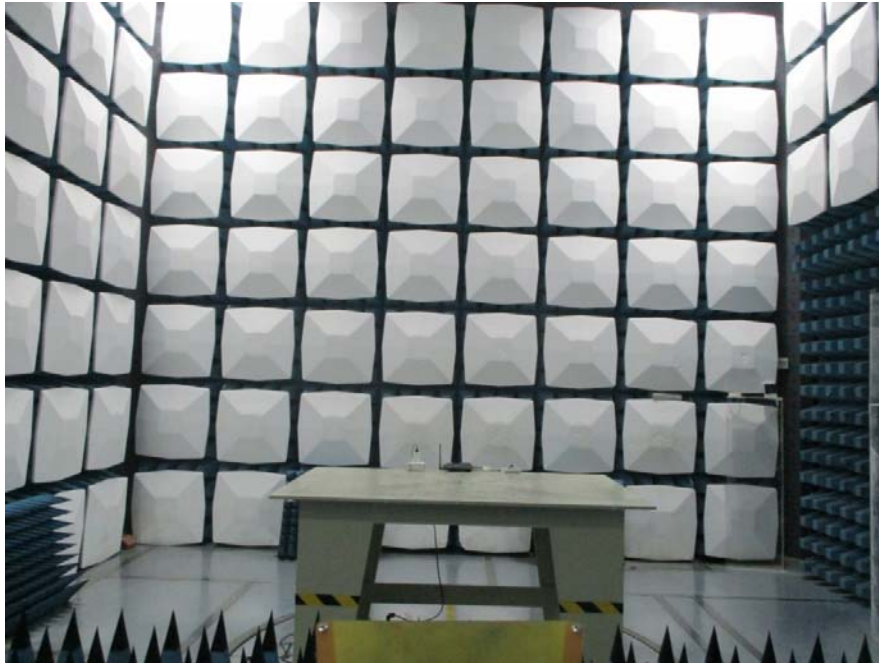
RE Above 1G Front View(USB Charging and Operating)
