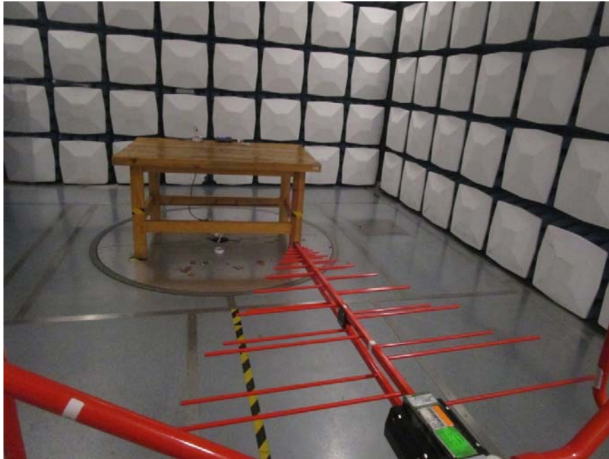
RE Below 1G Front View(USB Charging and Operating)
