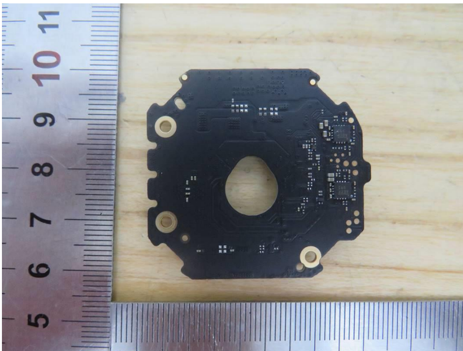
EUT Internal Photo 8
