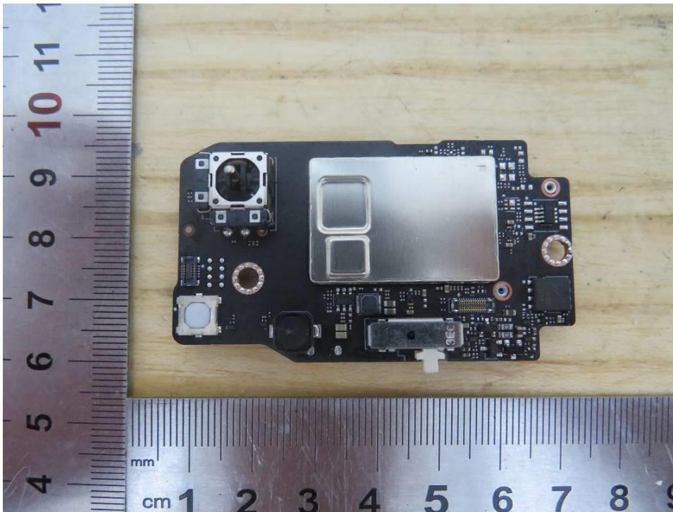
EUT Internal Photo 12
