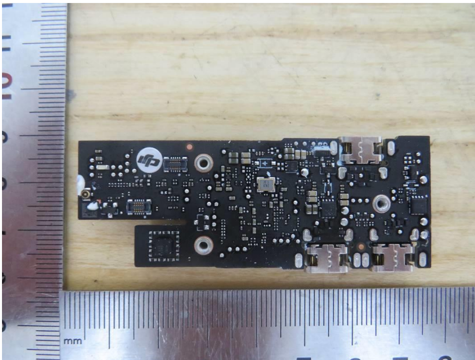
EUT Internal Photo 14
