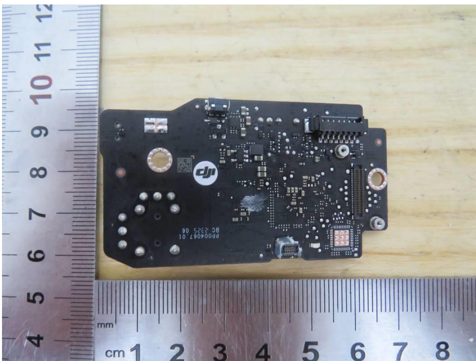
EUT Internal Photo 10
