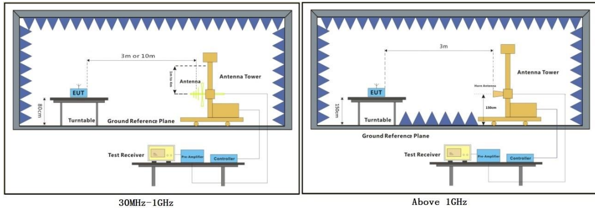
30MHz-1GHz
