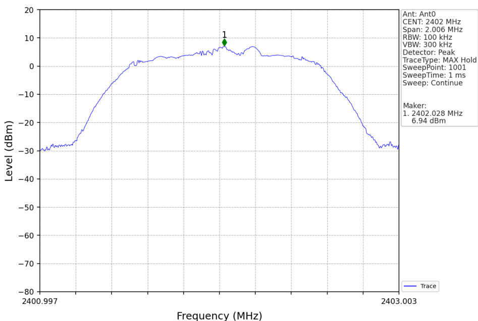
Pi/4DQPSK_2DH5_LCH_2402MHz_Ant0_NTNV
