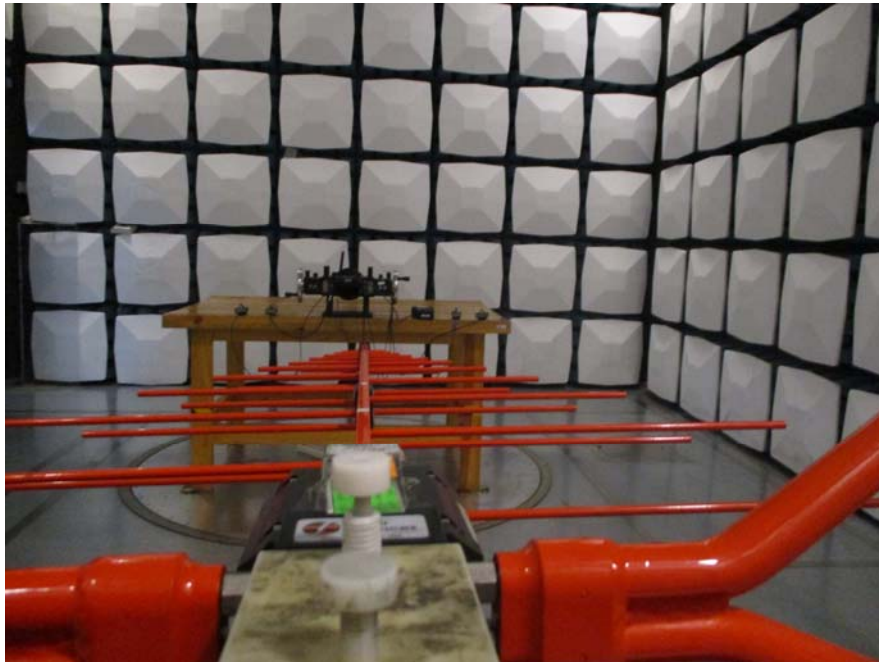
RE Below 1G Rear View for M2
