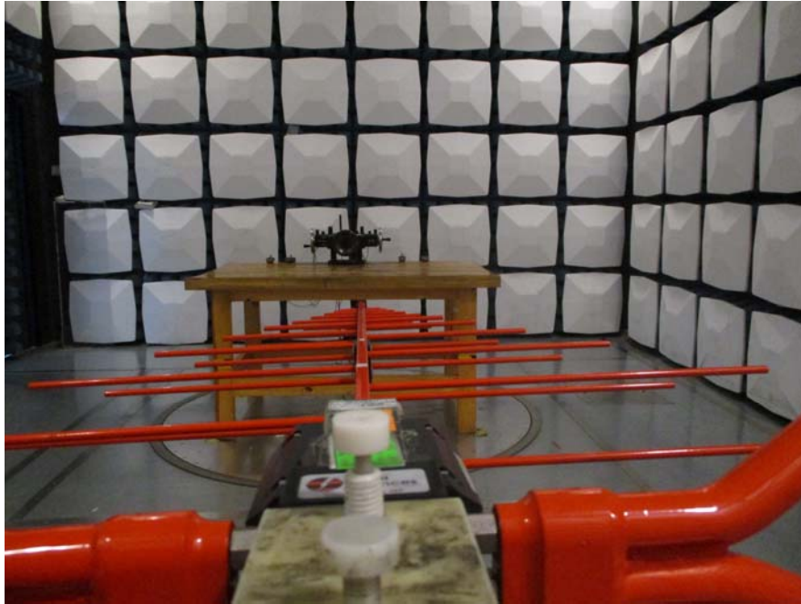
RE Below 1G Front View for M1
