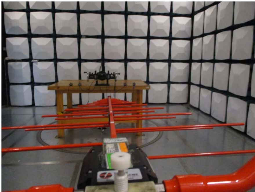
RE Below 1G Rear View for M1
