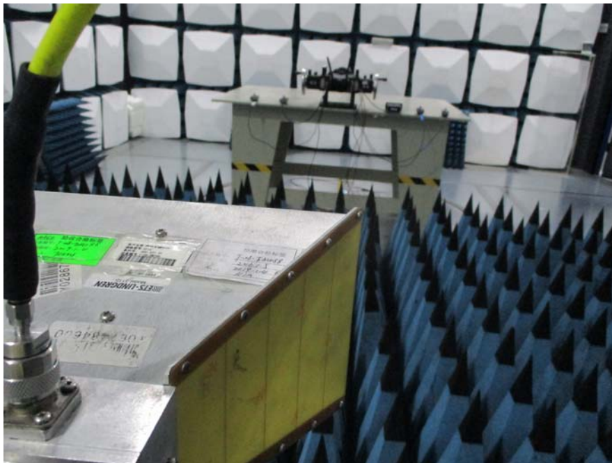
RE Above 1G Rear View for M2
