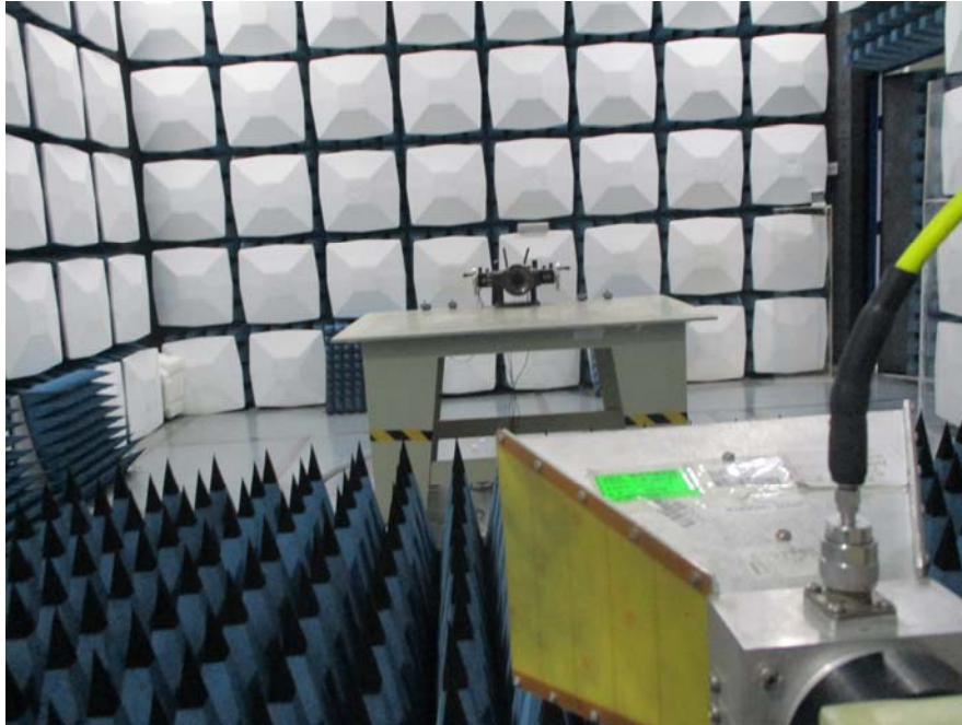
RE Above 1G Front View for M1
