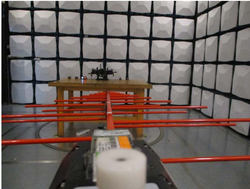
RE Below 1G Front View for M2
