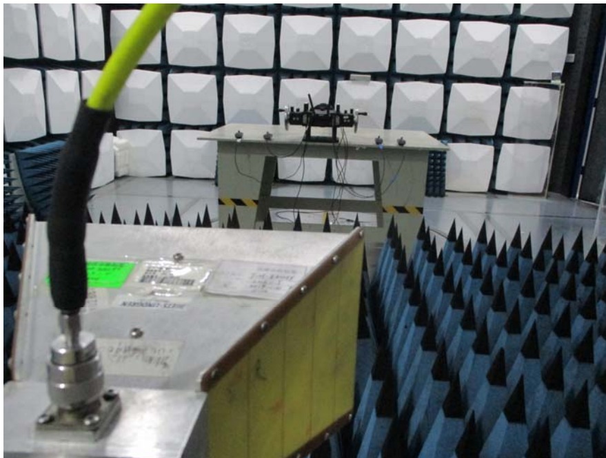
RE Above 1G Rear View for M1
