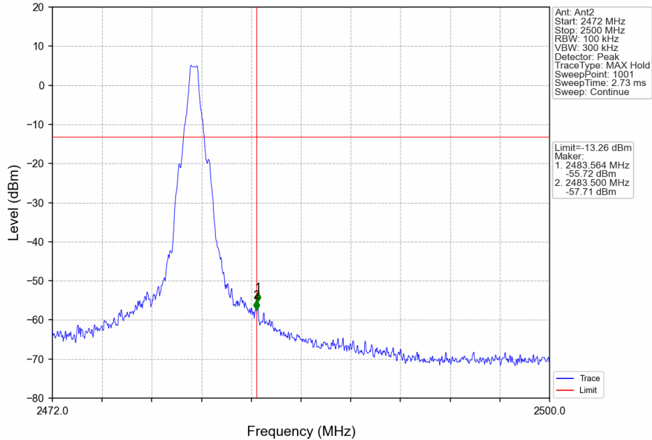
GFSK_DH5_HCH_2480MHz_Ant2_NTNV
