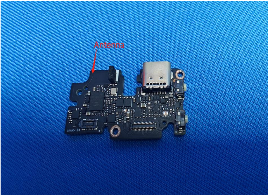
Antenna Location
