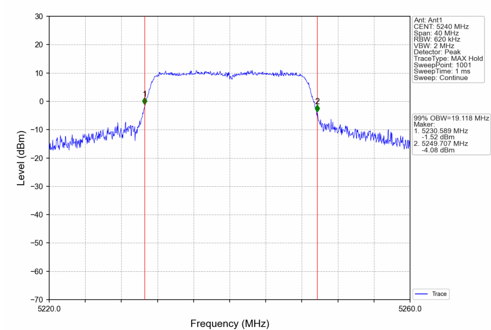
802.11n(HT20)_HCH_5240MHz_Ant1_NTNV
