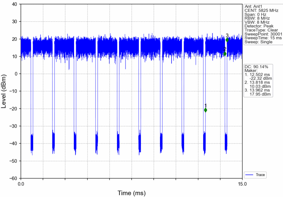
802.11ac(VHT20)_HCH_5825MHz_Ant1_NTNV
