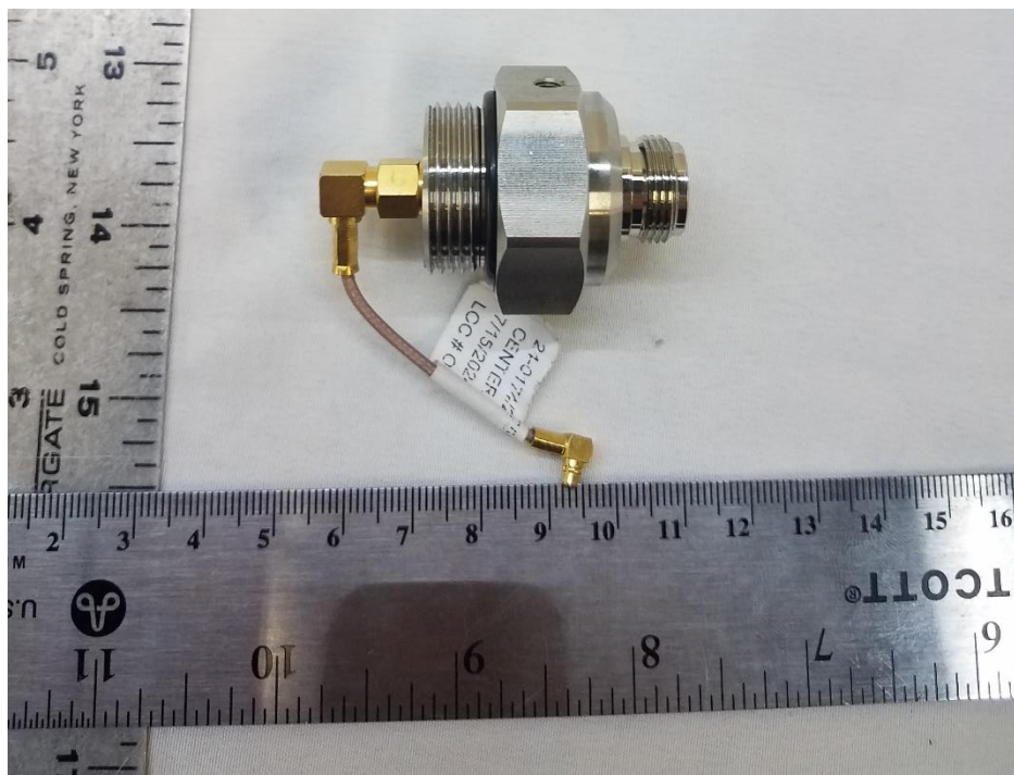
Figure 5. Connector Used for Antenna 2 - 4
