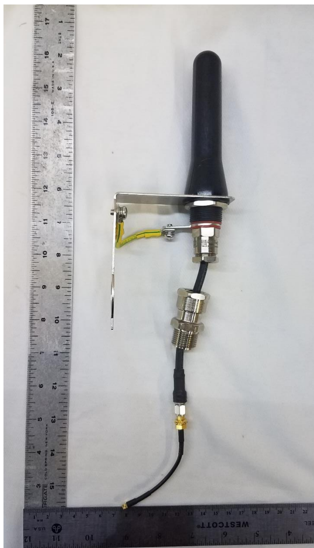
Figure 6. Antenna 5
