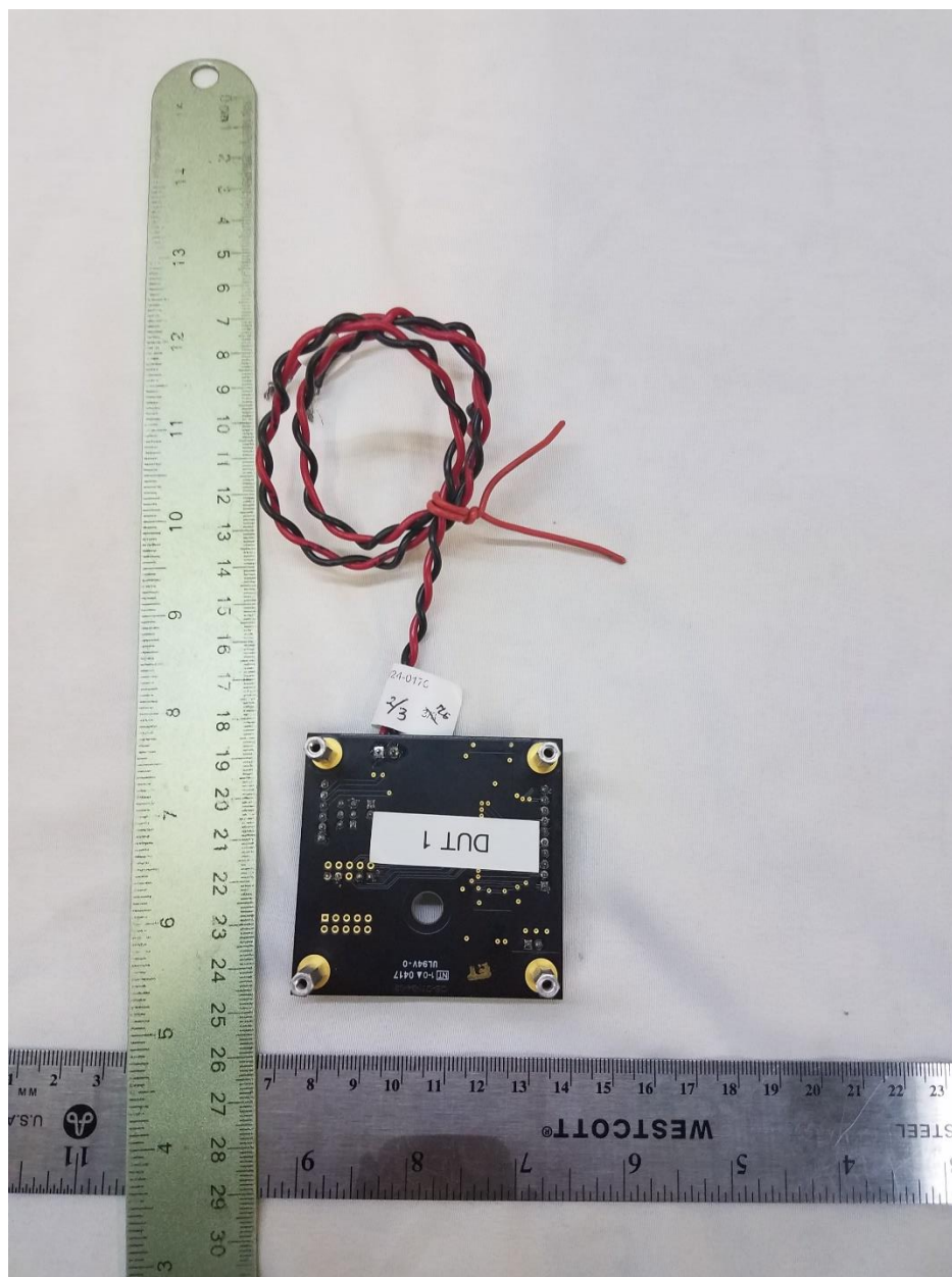
Figure 2. Bottom of Evaluation board
