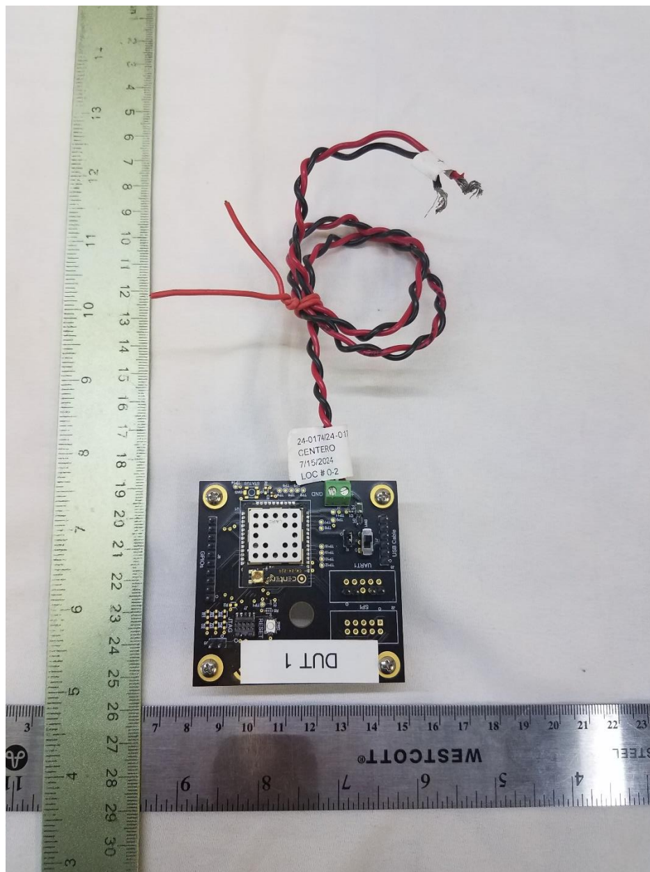
Figure 1. Top of Evaluation with EUT mounted
