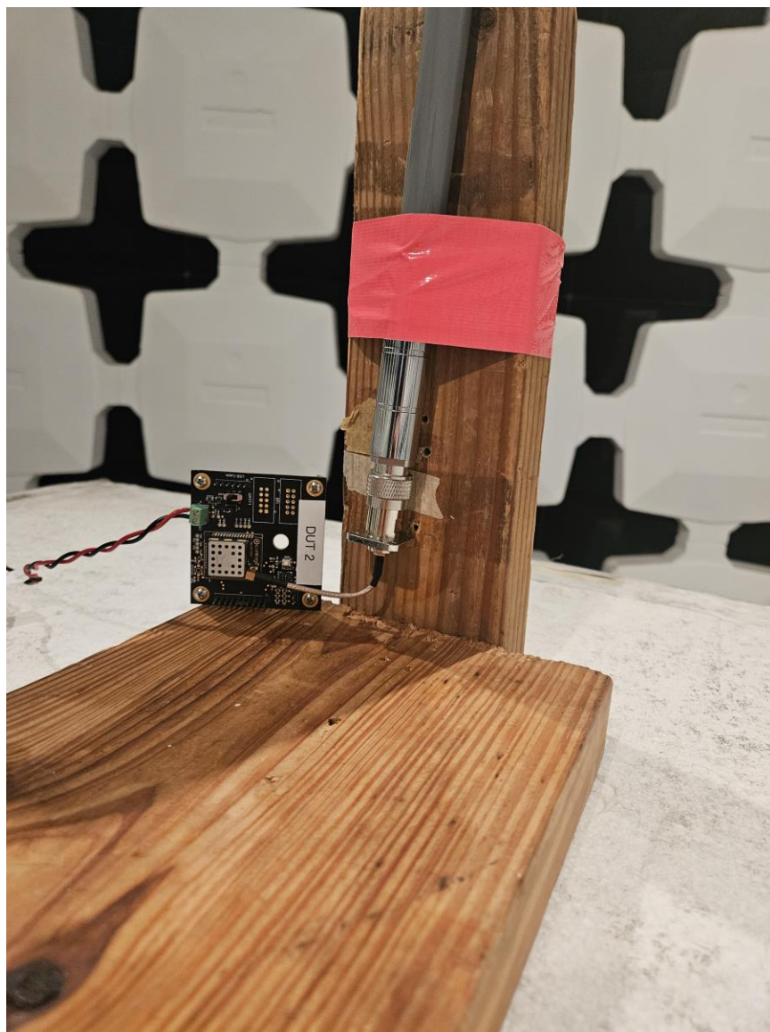
Figure 1. Radiated Emissions Test Setup, Front
