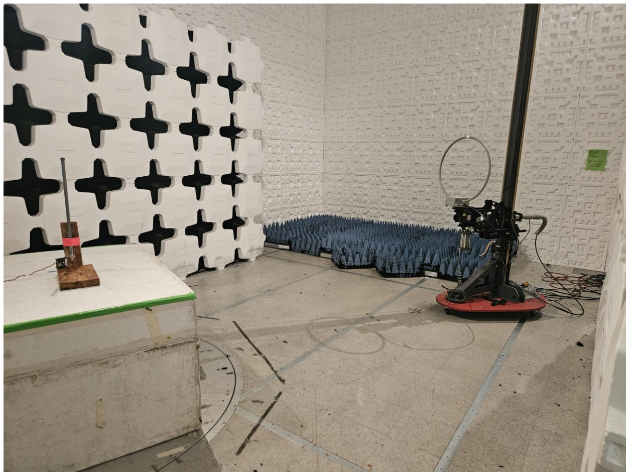
Figure 2. Radiated Emissions Test Setup, .15 MHz to 300 MHz
