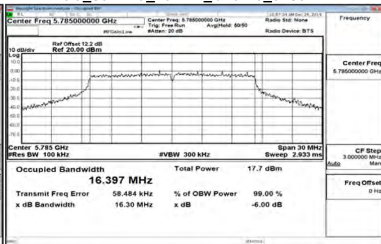
FCC_802.11a_20MHz_Chain0_5785MHz
