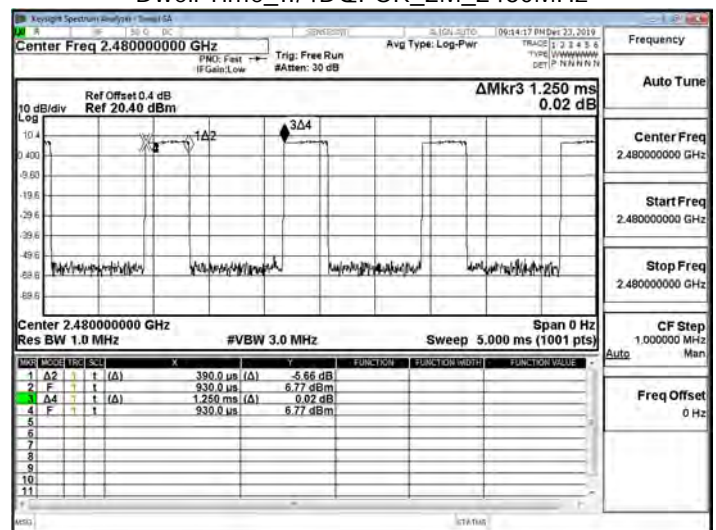
Dwell Time_π/4QPSK_2M_2480MHz
