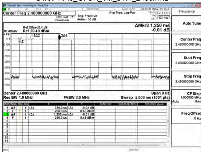
Dwell Time_GFSK_1M_DH1_2480MHz
