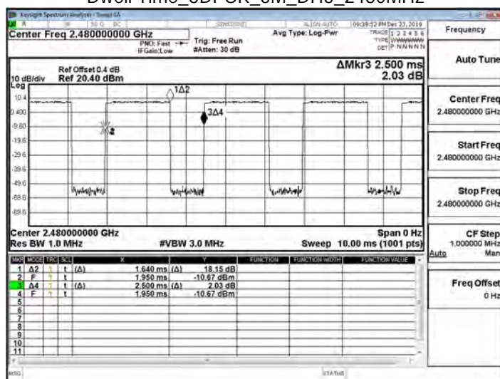
Dwell Time_8DPSK_3M_DH3_2480MHz
