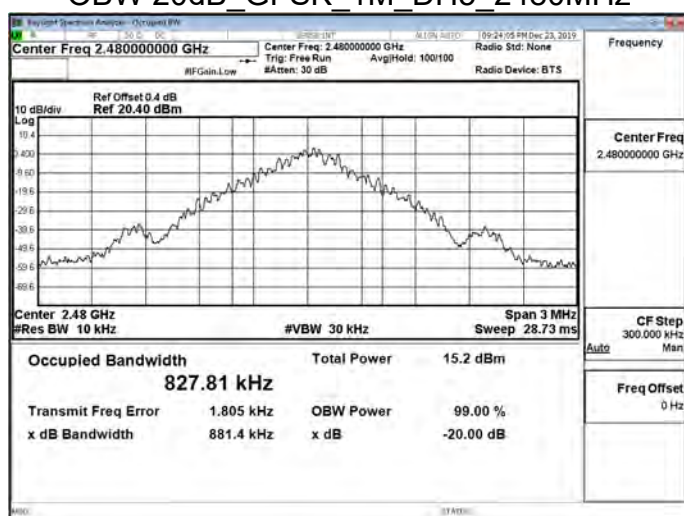
OBW 20dB_GFSK_1M_DH5_2480MHz
