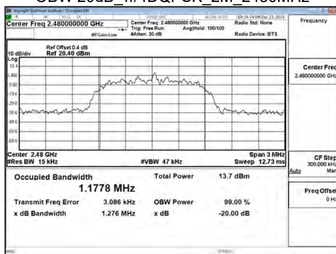
OBW 20dB_π/4DQPSK_2M_2480MHz
