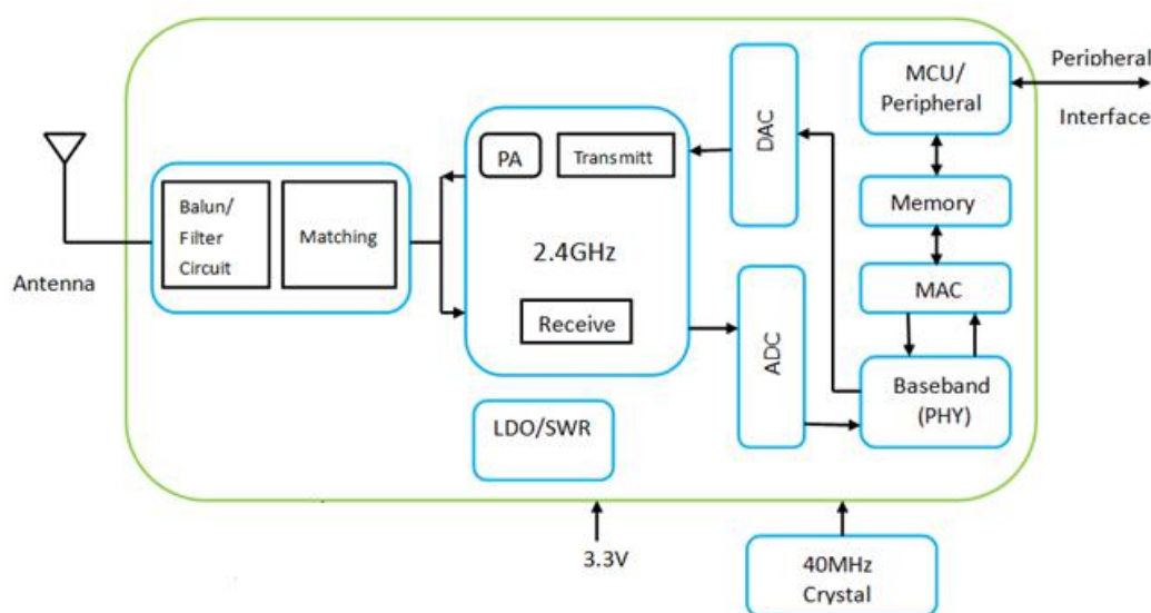
Figure 1-1 WBR3 architecture
