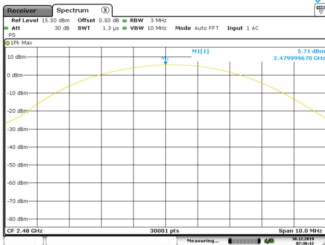
Channel 39 (2480MHz)
