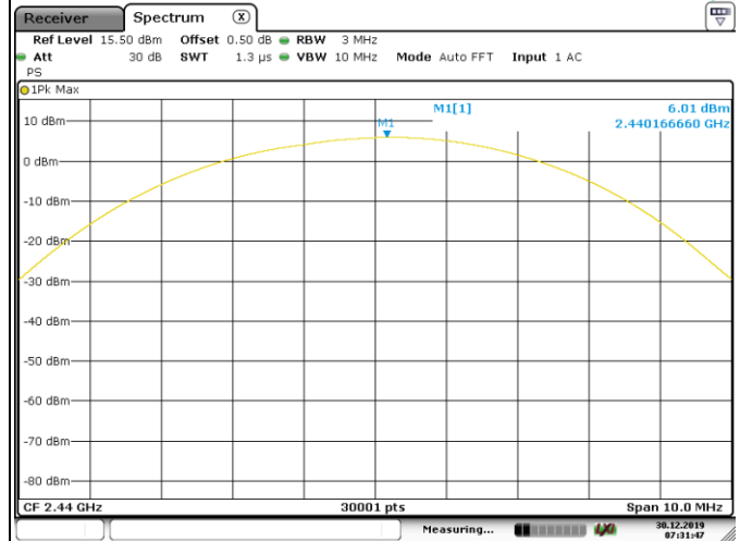
Channel 19 (2440MHz)
