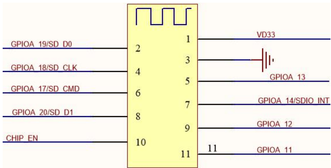
Figure 6-2 WBR2 pins
