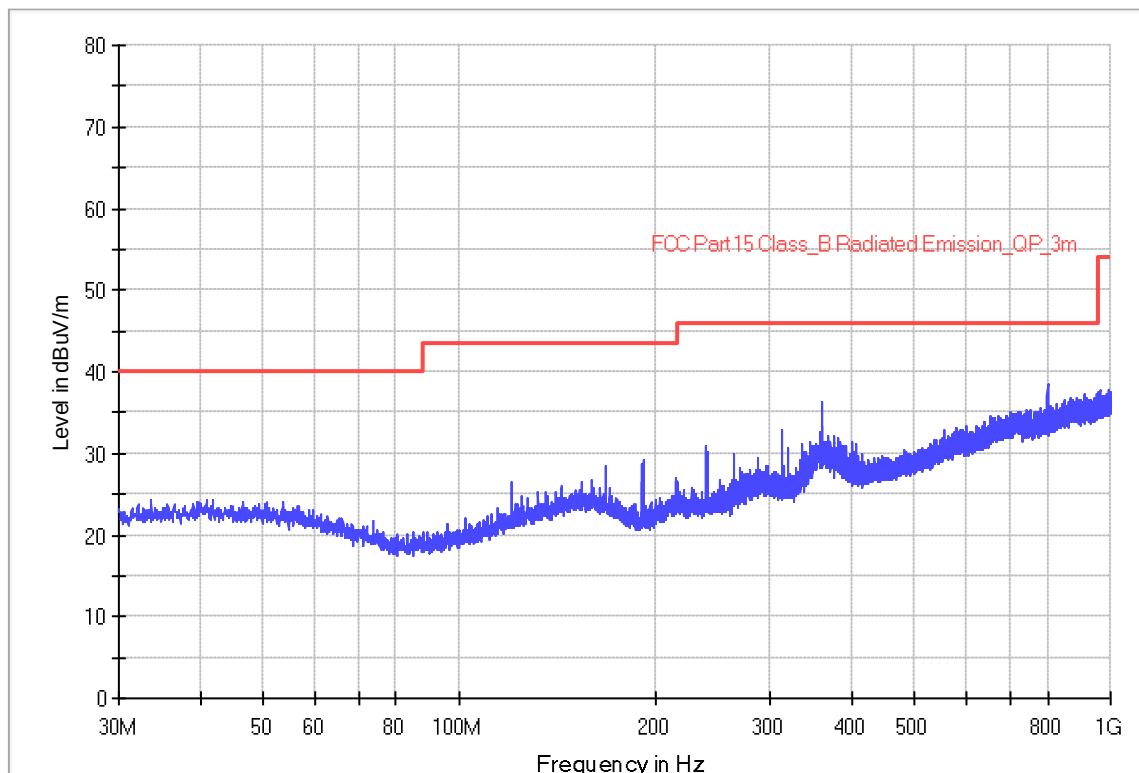
RE_VULB9168_pre_Conf_30-1000
