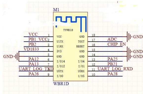
Figure 7-3 WBR1D pins
