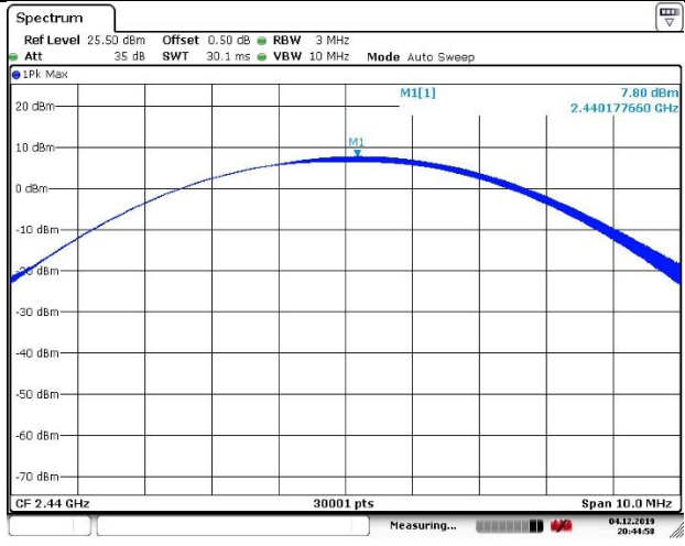
Channel 19 (2440MHz)
