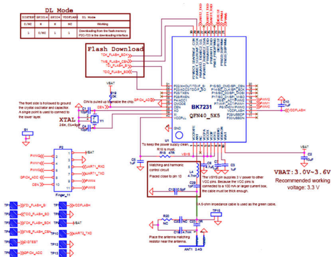
Figure 7-1 WB2S schematic diagram
