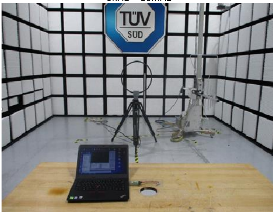
Radiated Emission Setup 9kHz ~ 30MHz
