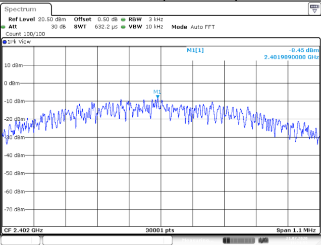
Channel 0 (2402MHz)
