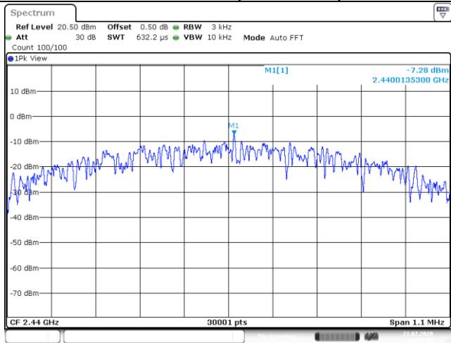
Channel 19 (2440MHz)
