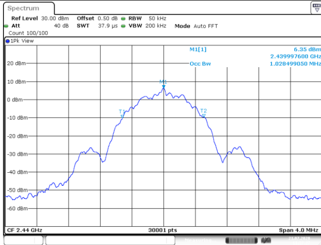
Channel 19 (2440MHz)
