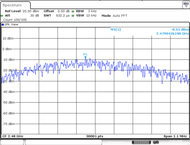
Channel 39 (2480MHz)
