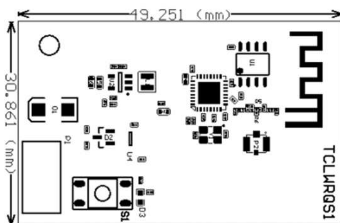
Figure 1 TCLWRQS1 front views
