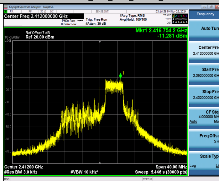
11AX20SISO_Ant1_2412_52Tone_RU40
