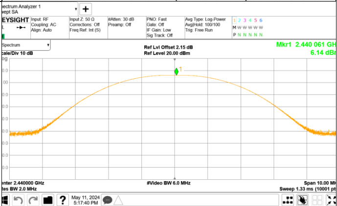
Channel 19 (2440MHz)
