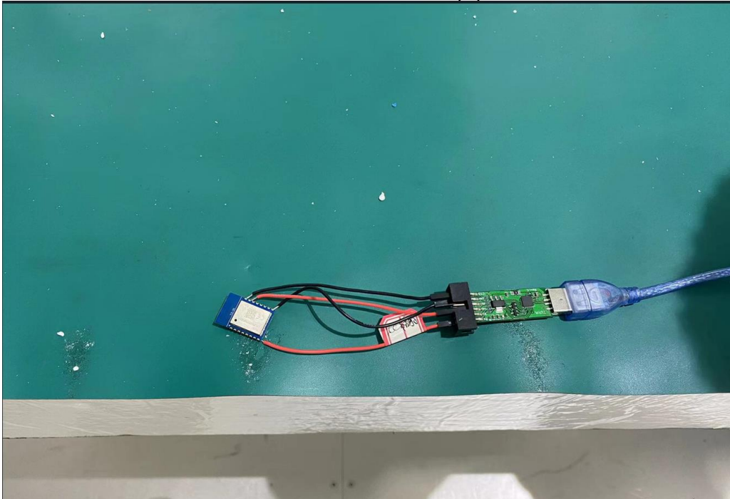
Radiated emission close-up photo
