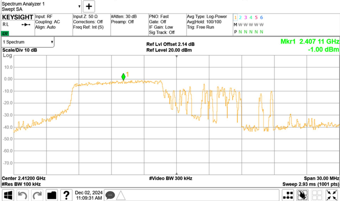
Band Edge NVNT ax20 2412MHz Ant1 Emission RU106_53
