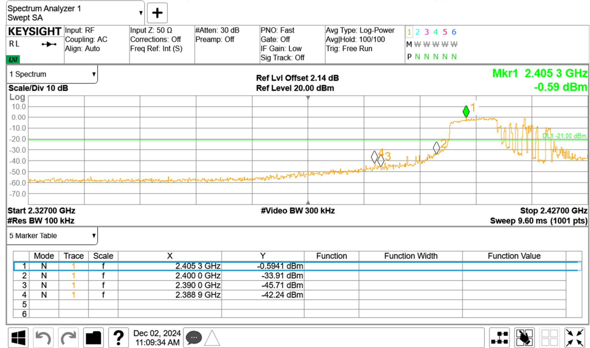
Band Edge NVNT ax20 2412MHz Ant1 Emission RU106_53
