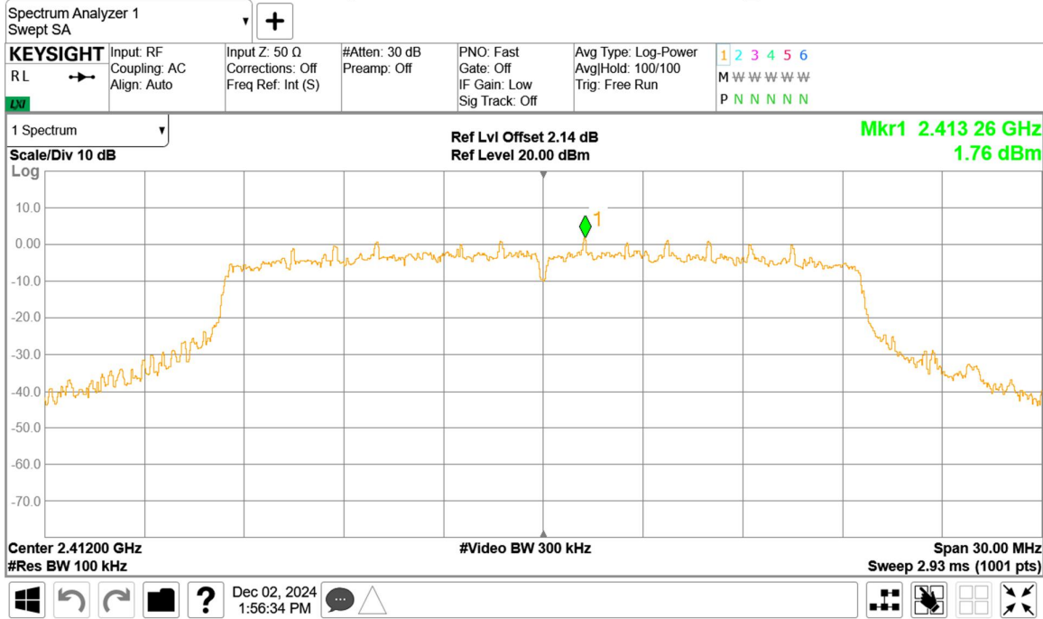
Band Edge NVNT ax20 2412MHz Ant1 Emission RU242_61
