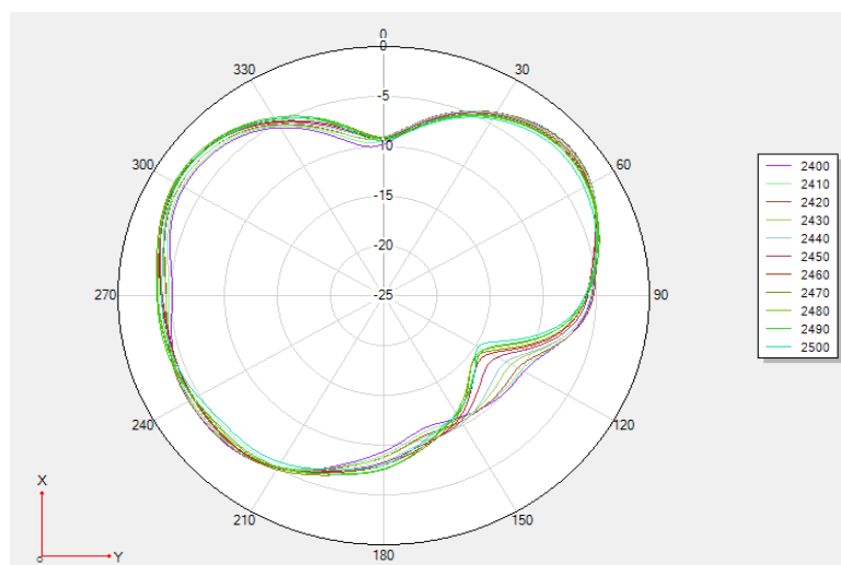
Theta 90 2D
