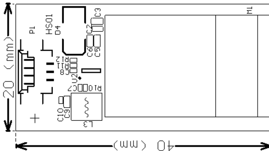
Figure 3 HS01 mechanical dimension
