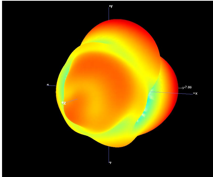
B1.1 3D Pattern for 2404MHz
