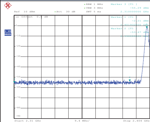
Channel 0 / 2402 MHz – Peak
