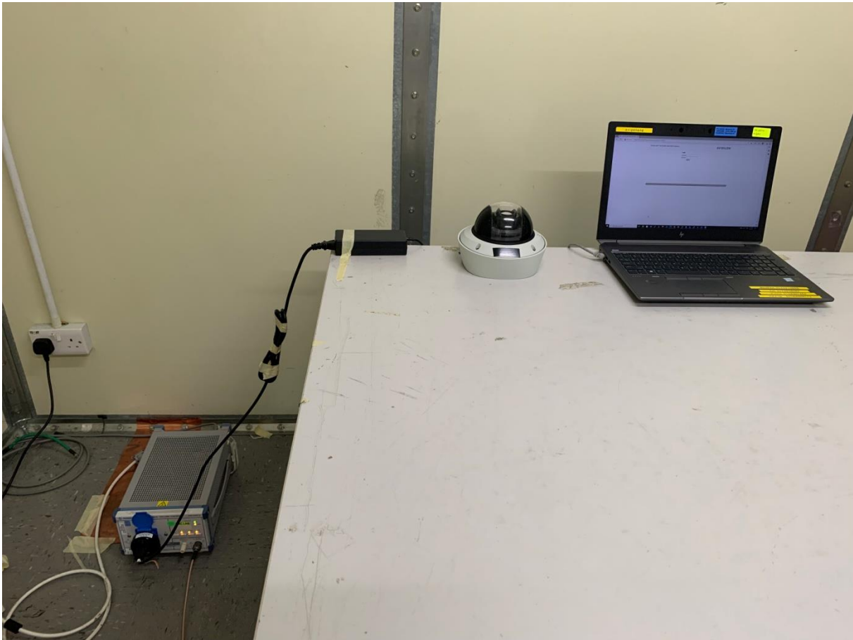
Conducted Emission Test Setup Photo
