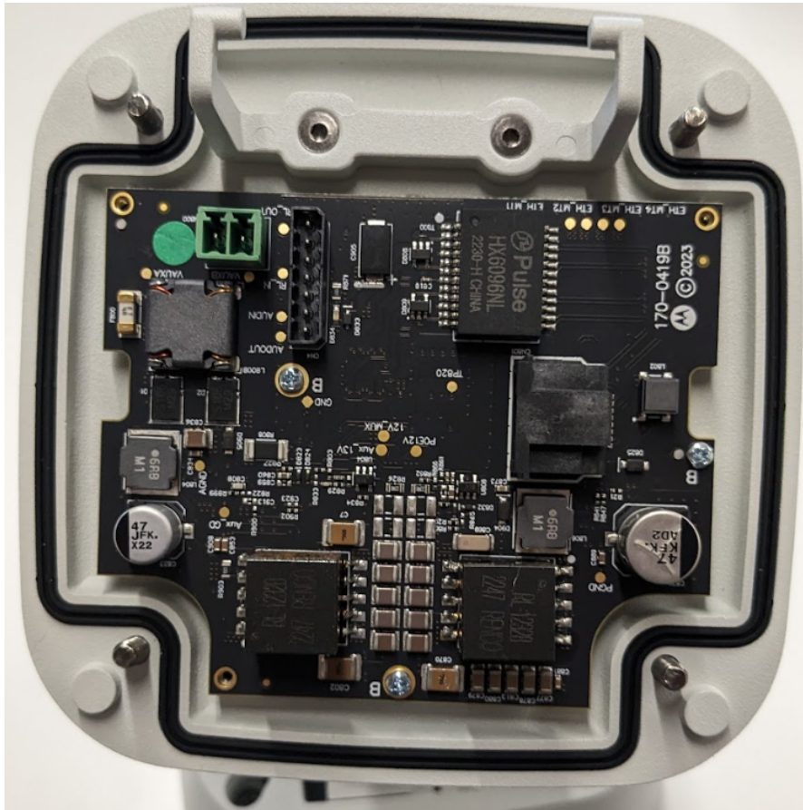
Internal Photo: Power Board in Base Pan
