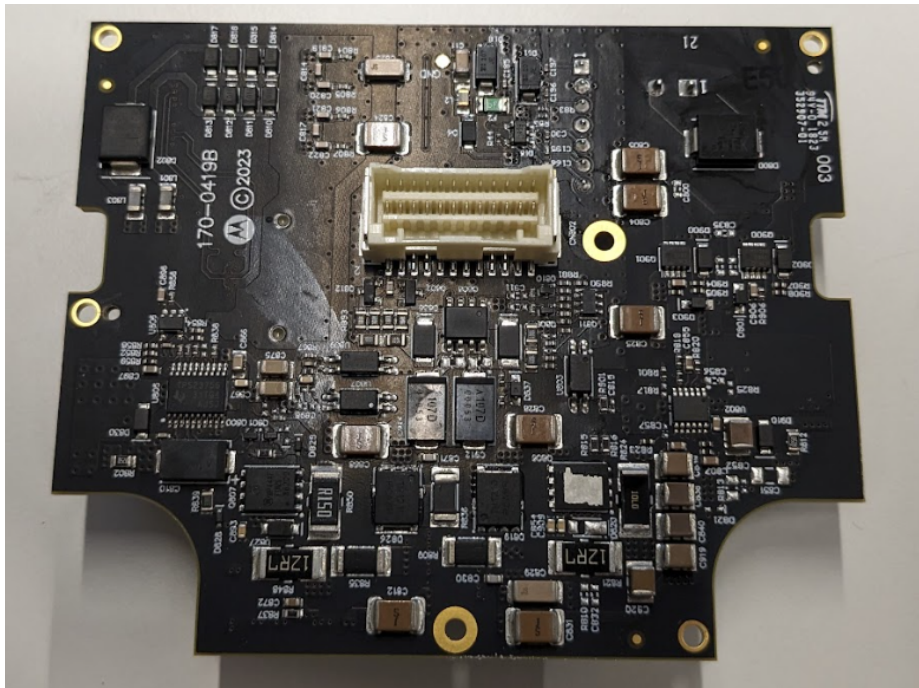
Internal Photo: Power Board Bottom
