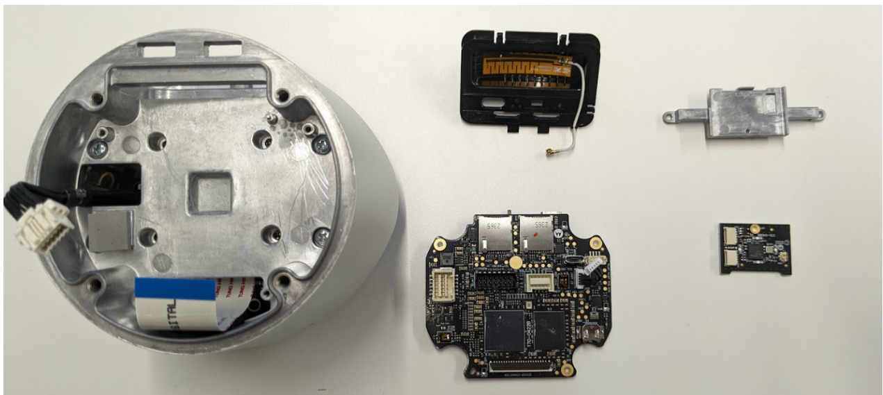
Internal Photo: Mainboard Top with Base Pan, IoT Hub Board & RF Antenna Shroud
