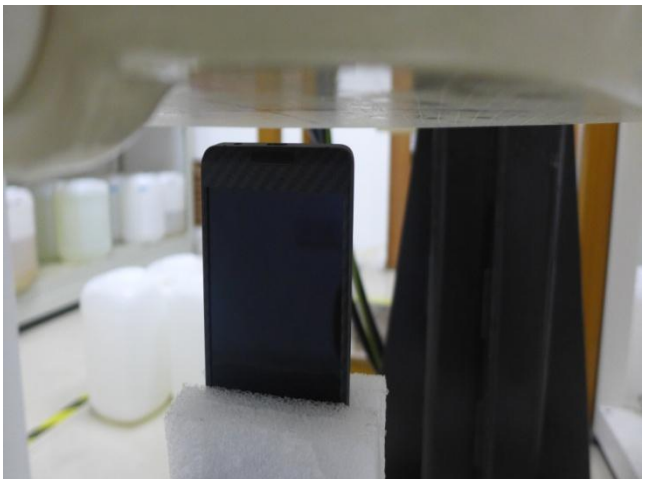
Photo 24: Bottom side 10mm
