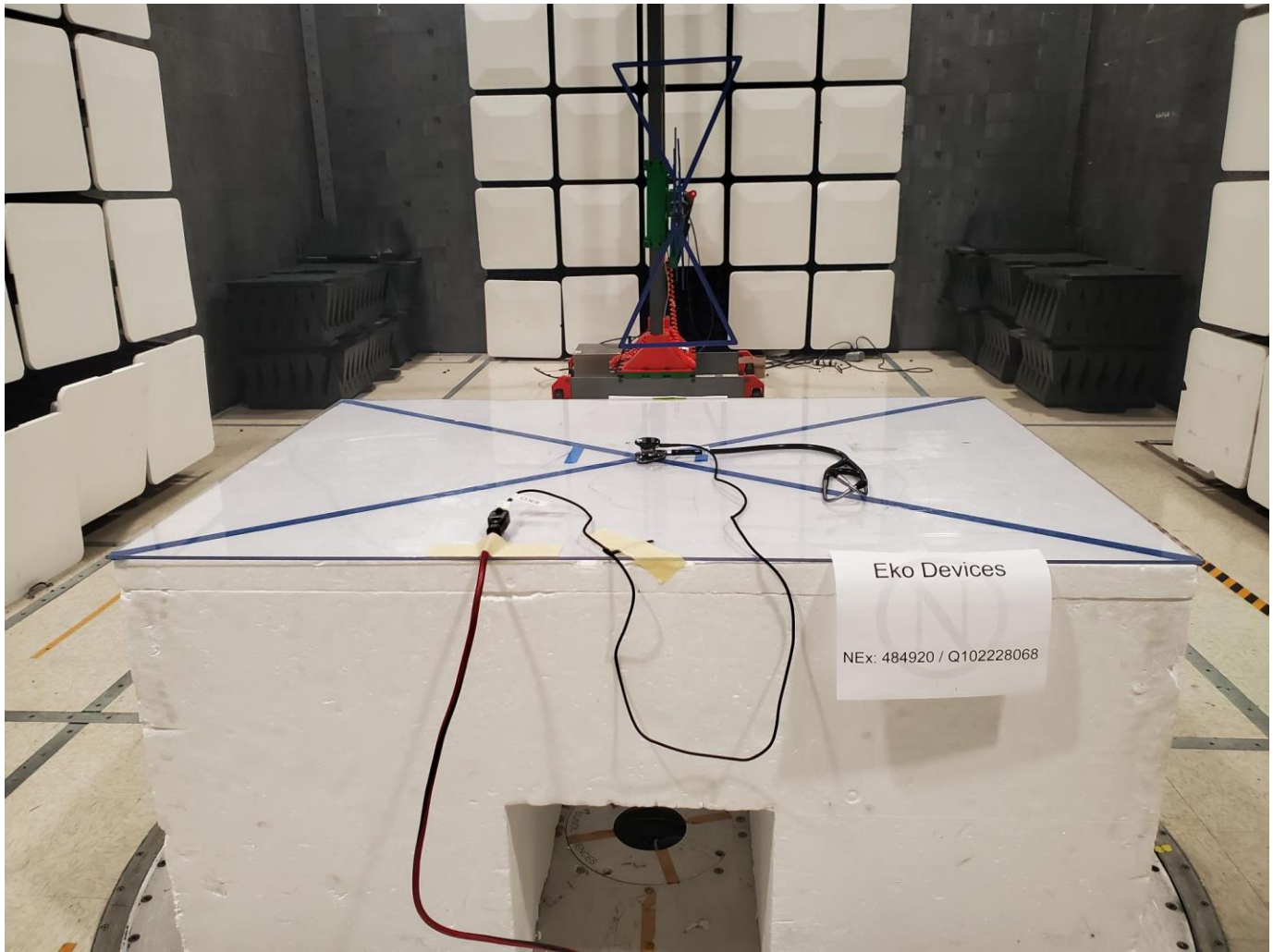
Figure 4 - Radiated emissions below 1 GHz (0.03 – 1 GHz), rear view.
