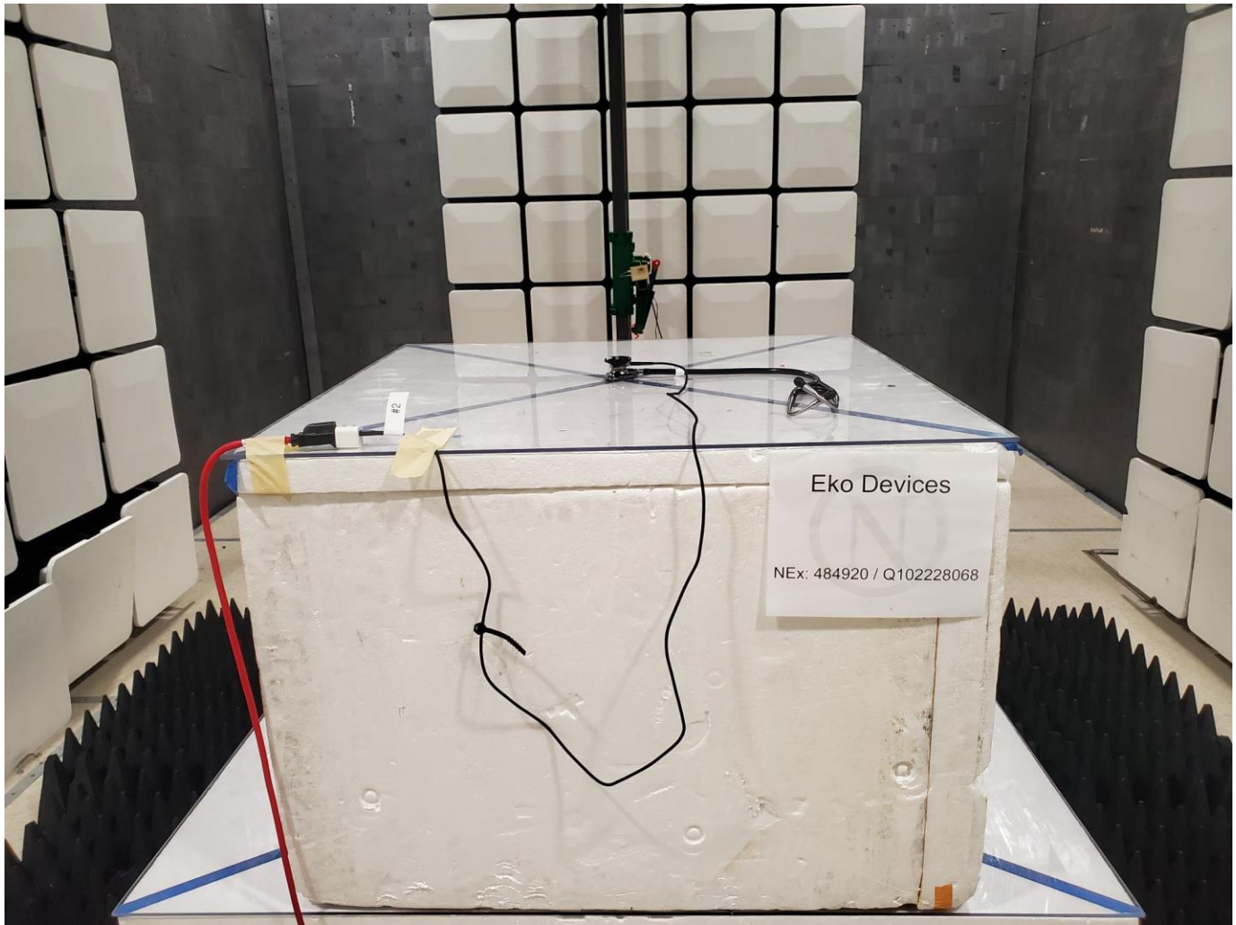
Figure 8 - Radiated emissions above 1 GHz (18 – 26 GHz).
