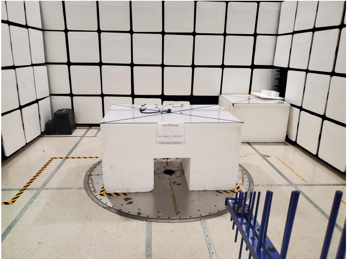
Figure 3 - Radiated emissions below 1 GHz (0.03 – 1 GHz), front view.
