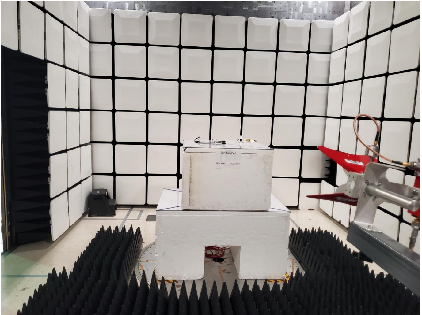
Figure 5 - Radiated emissions above 1 GHz (1 – 18 GHz), front view.
