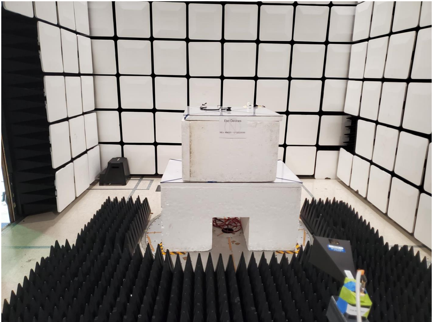
Figure 7 - Radiated emissions above 1 GHz (18 – 26 GHz), front view.
