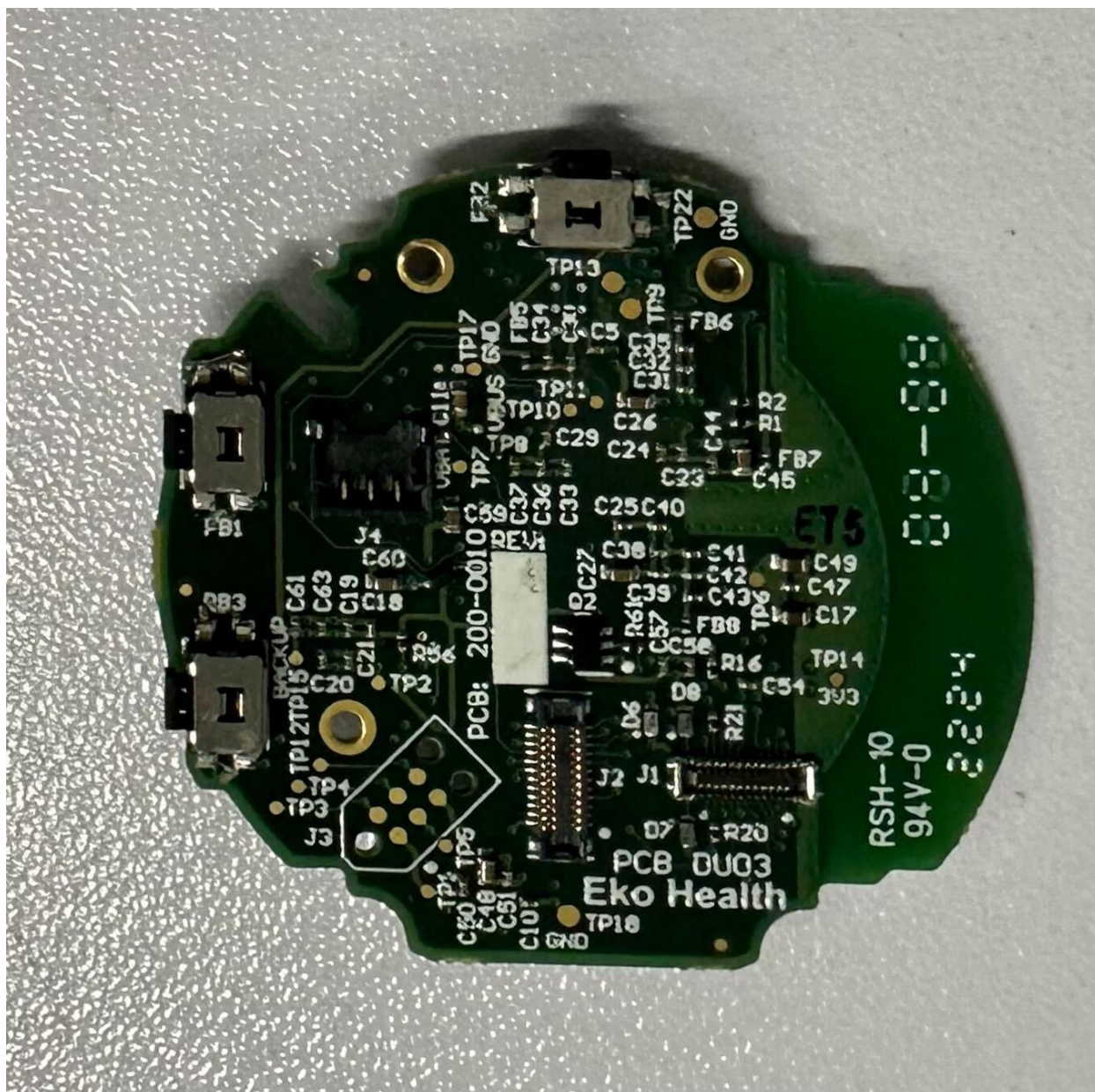
Mainboard Front View
