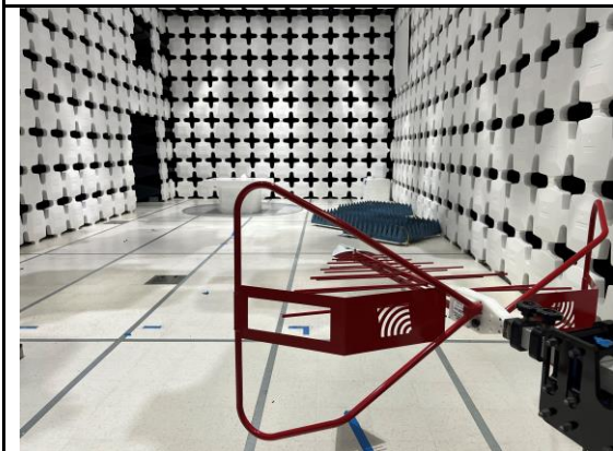
RE below 1GHz test - Front View
