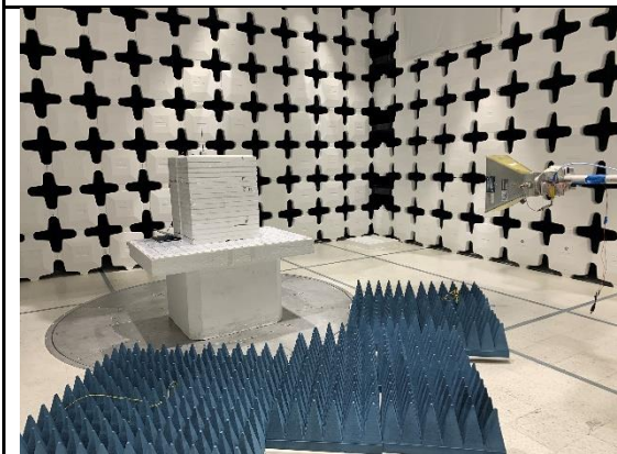
RE above 1GHz test - Front View
