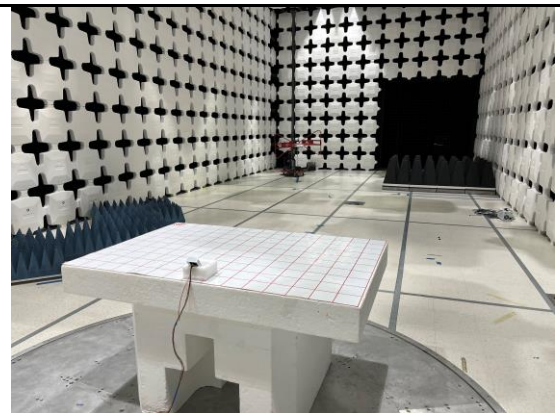
RE below 1GHz test - Rear View
