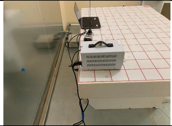
Conducted emission test - Rear View
