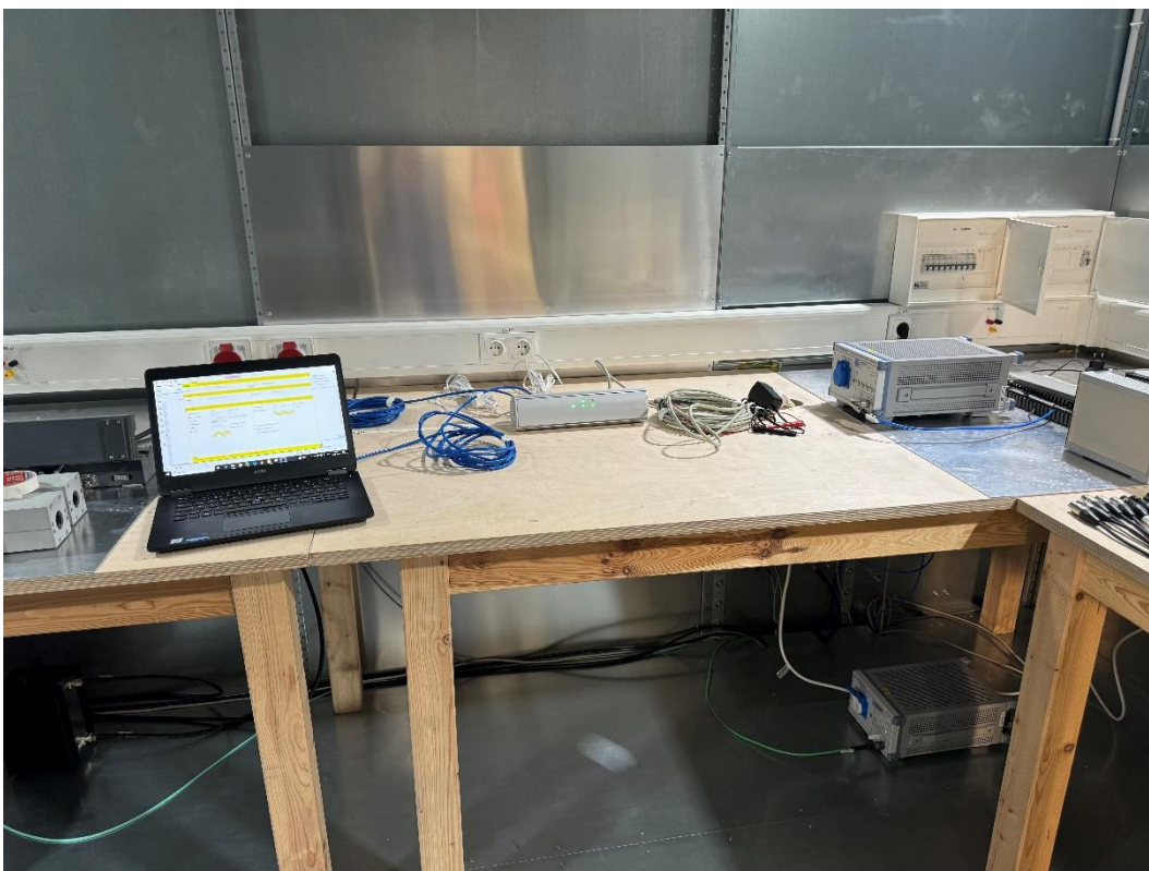
Photograph 10: Overall view, set-up 2.
