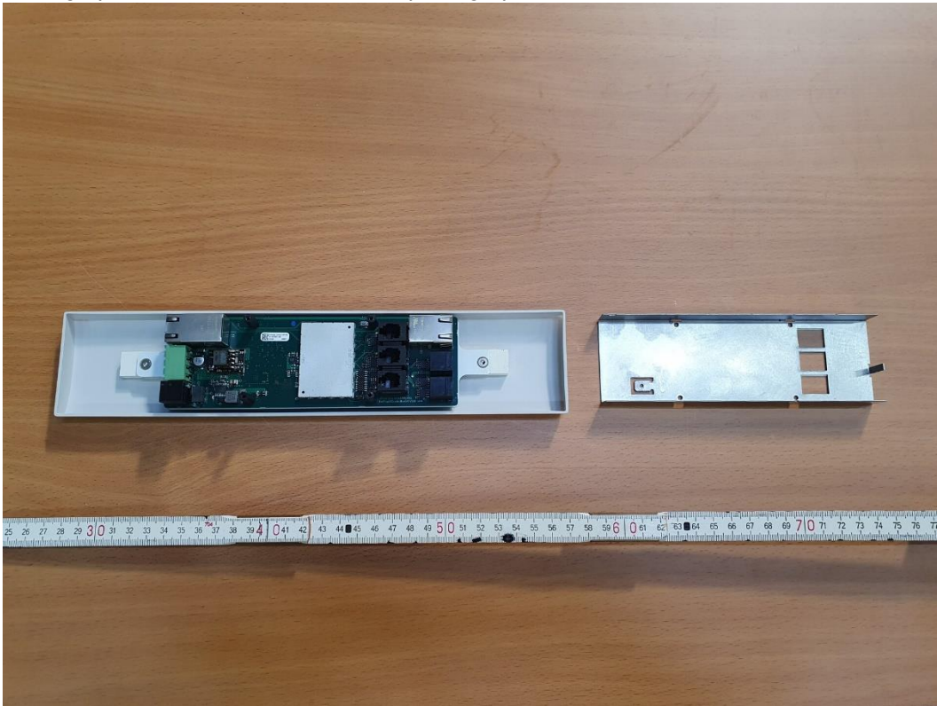
Photograph 4: View 2, EUT A, internal photograph
