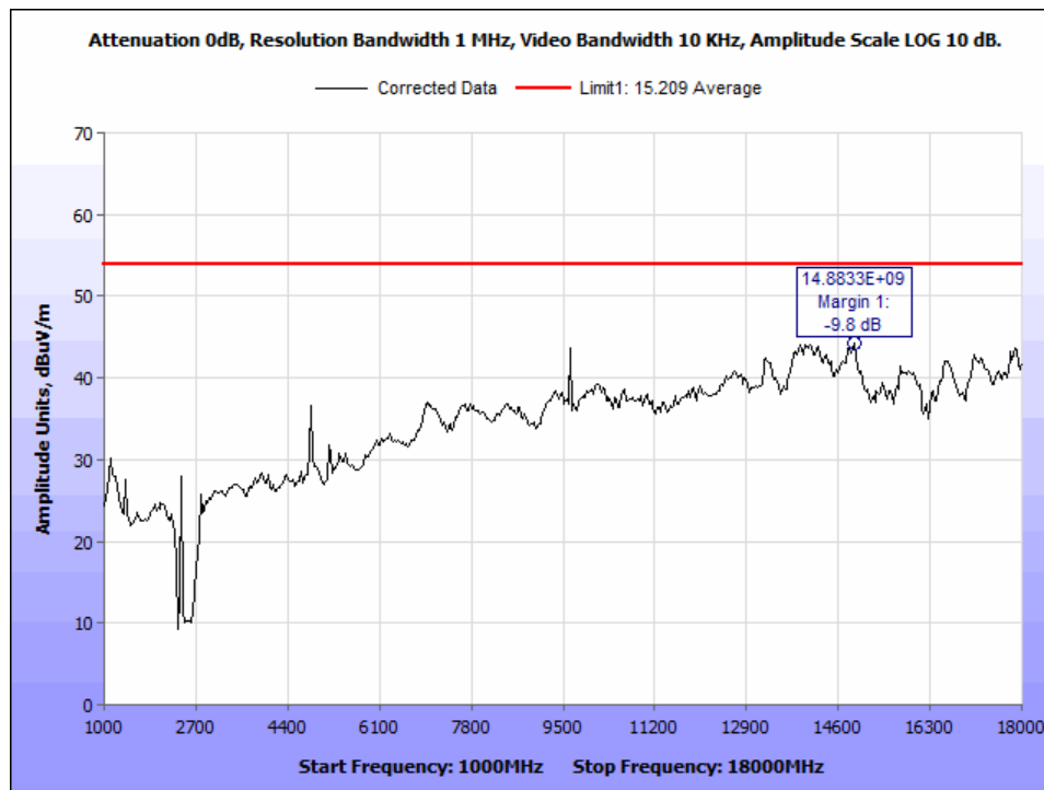
Figure 20: AVG_Radiated Emissions_802.11n20_2412Mz_1-18GHz.
