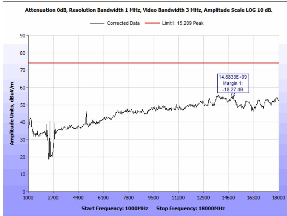
Figure 34: PK_Radiated Emissions_802.11n20_2462Mz_1-18GHz.
