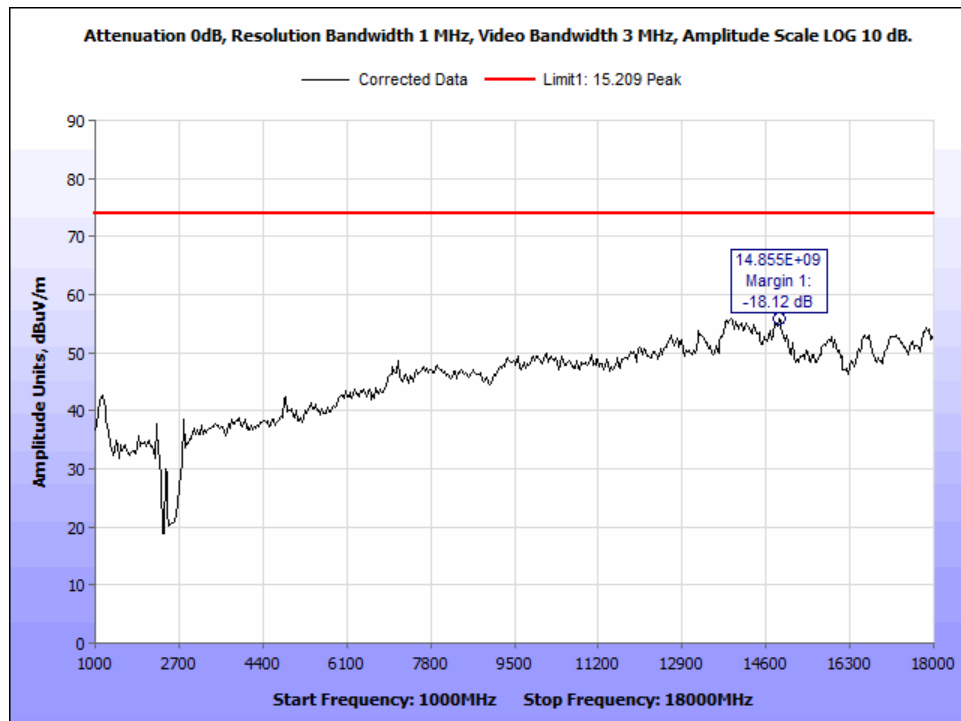
Figure 35: PK_Radiated Emissions_802.11n40_2422Mz_1-18GHz.
