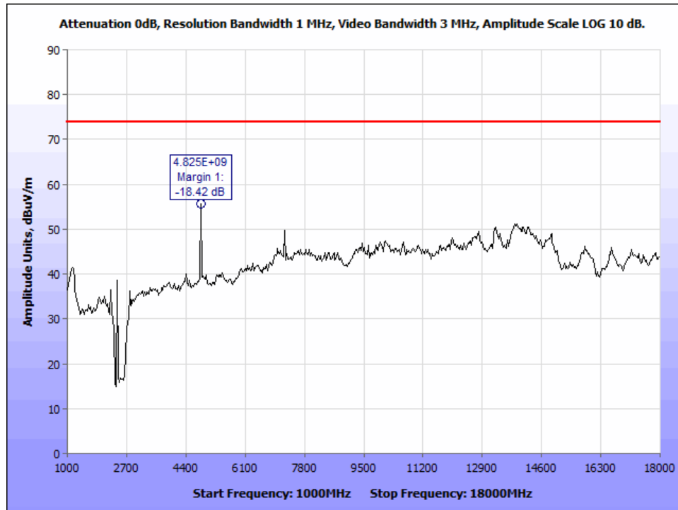
Figure 26: PK_Radiated Emissions_802.11b_2412Mz_1-18GHz.
