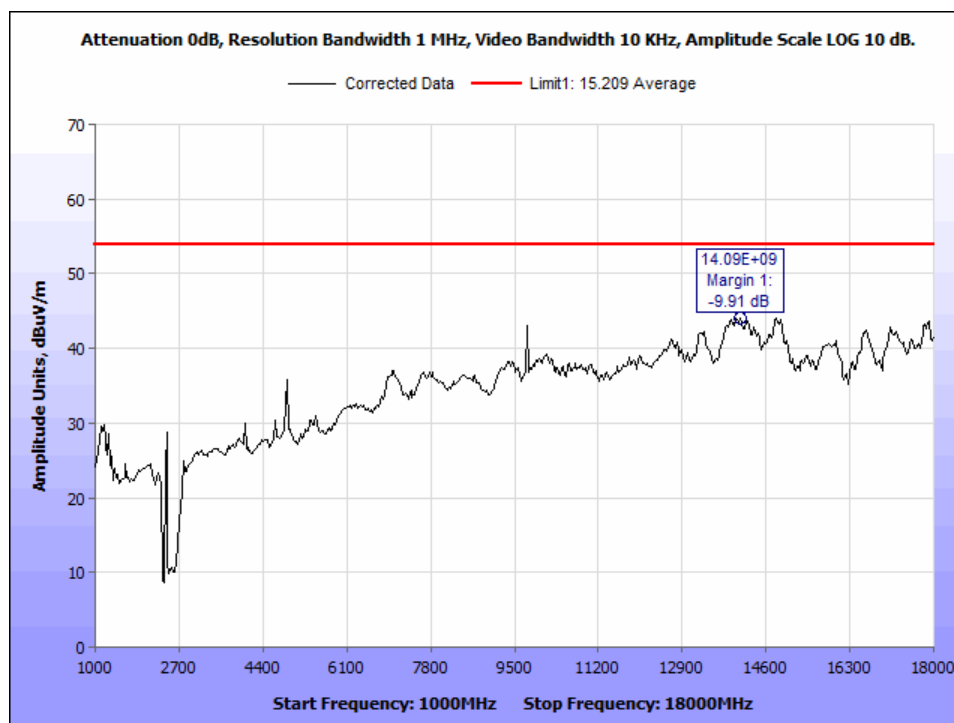
Figure 21: AVG_Radiated Emissions_802.11n20_2437Mz_1-18GHz.
