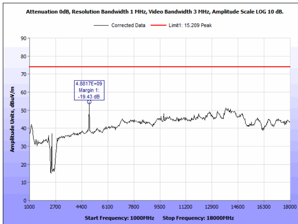
Figure 27: PK_Radiated Emissions_802.11b_2437Mz_1-18GHz.
