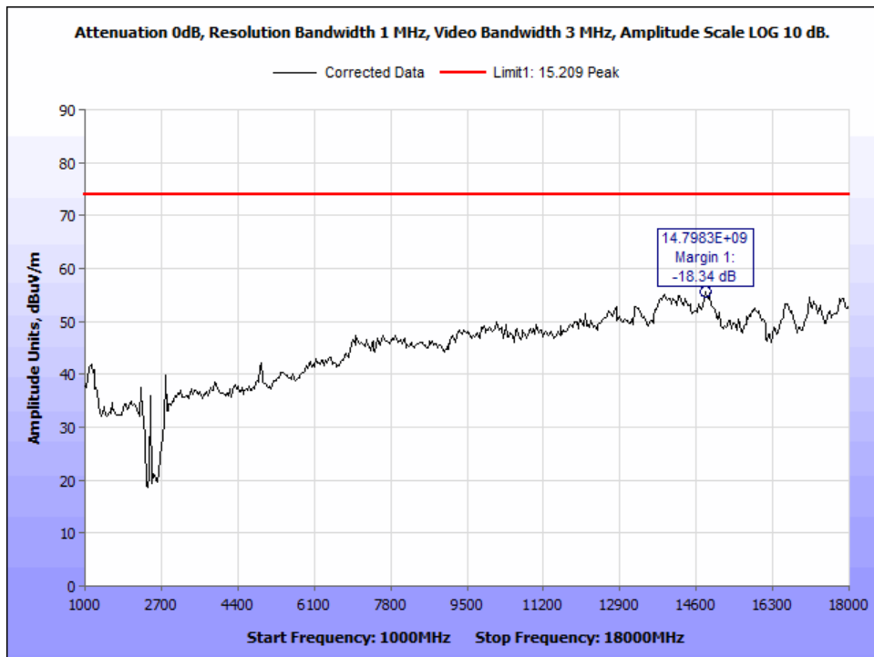
Figure 37: PK_Radiated Emissions_802.11n40_2452Mz_1-18GHz.
