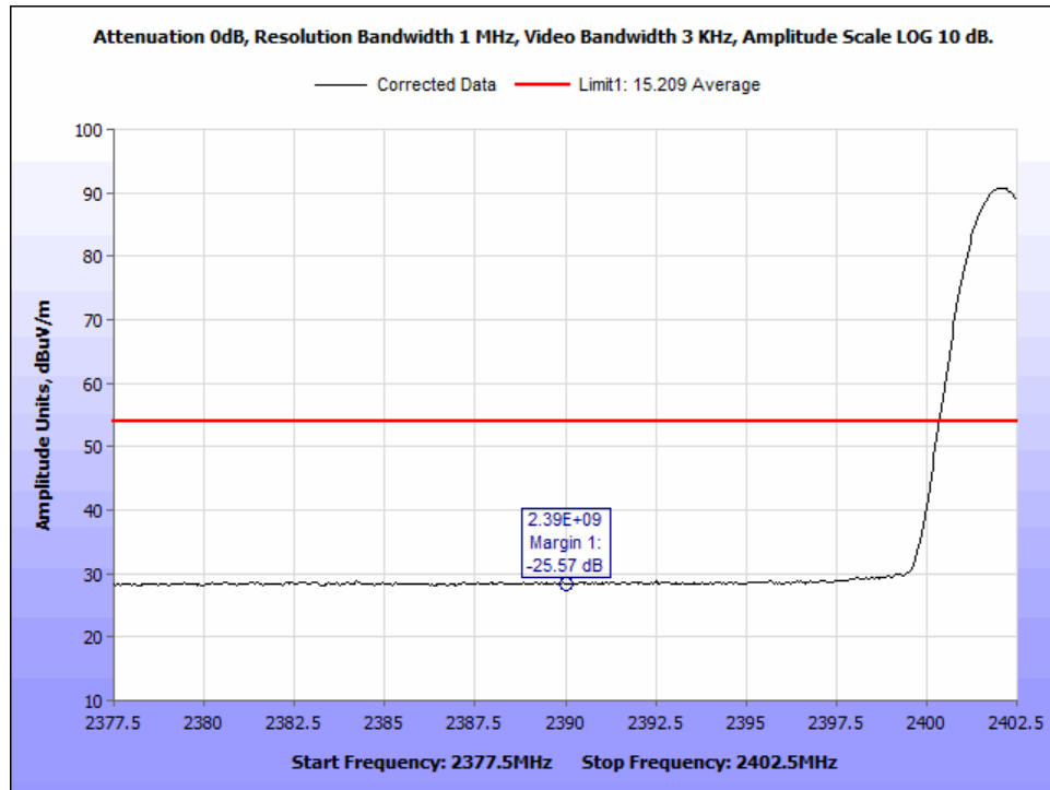
Figure 47: AVG_DH3_Radiated Band Edge_2390MHz_CF 2402 MHz.
