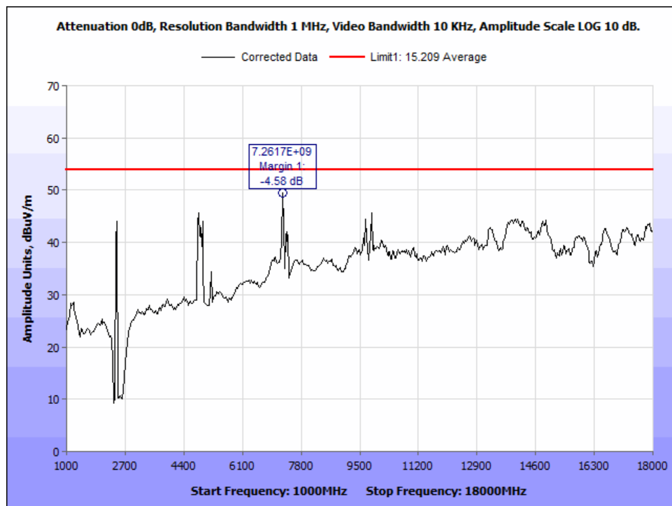
Figure 19: DH1_hopping_AVG Radiated Emissions_1-18 GHz.
