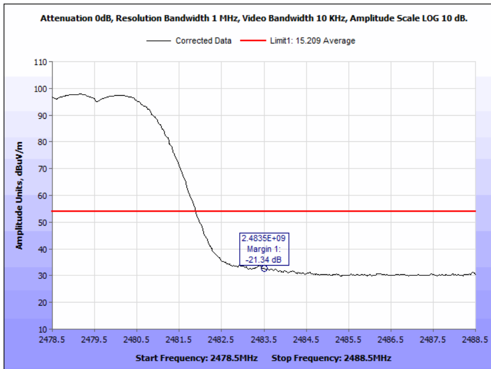
Figure 46: AVG_DH1_Radiated Band Edge_2483.5MHz_hopping.
