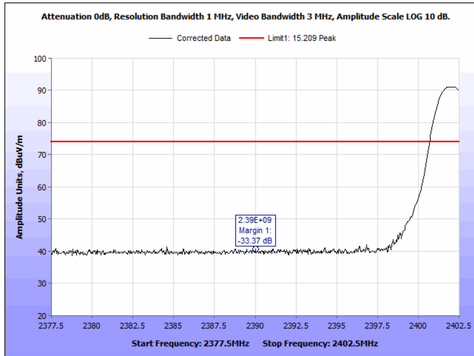
Figure 63: PK_DH5_Radiated Band Edge_2390MHz_CF 2402 MHz.
