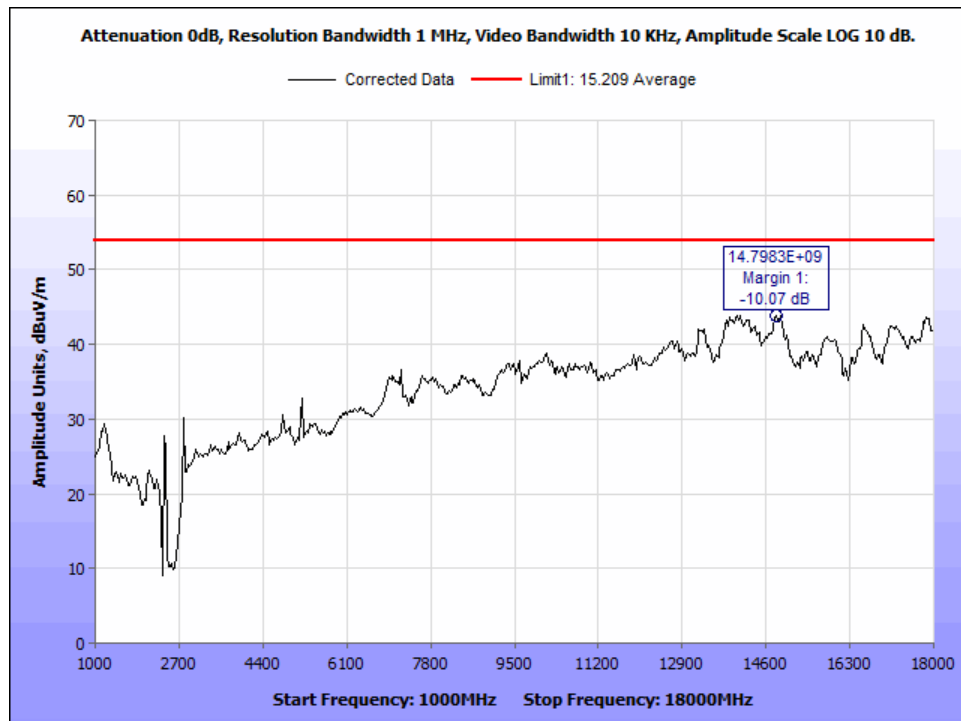
Figure 29: DH5_ch 2402_AVG Radiated Emissions_1-18 GHz.
