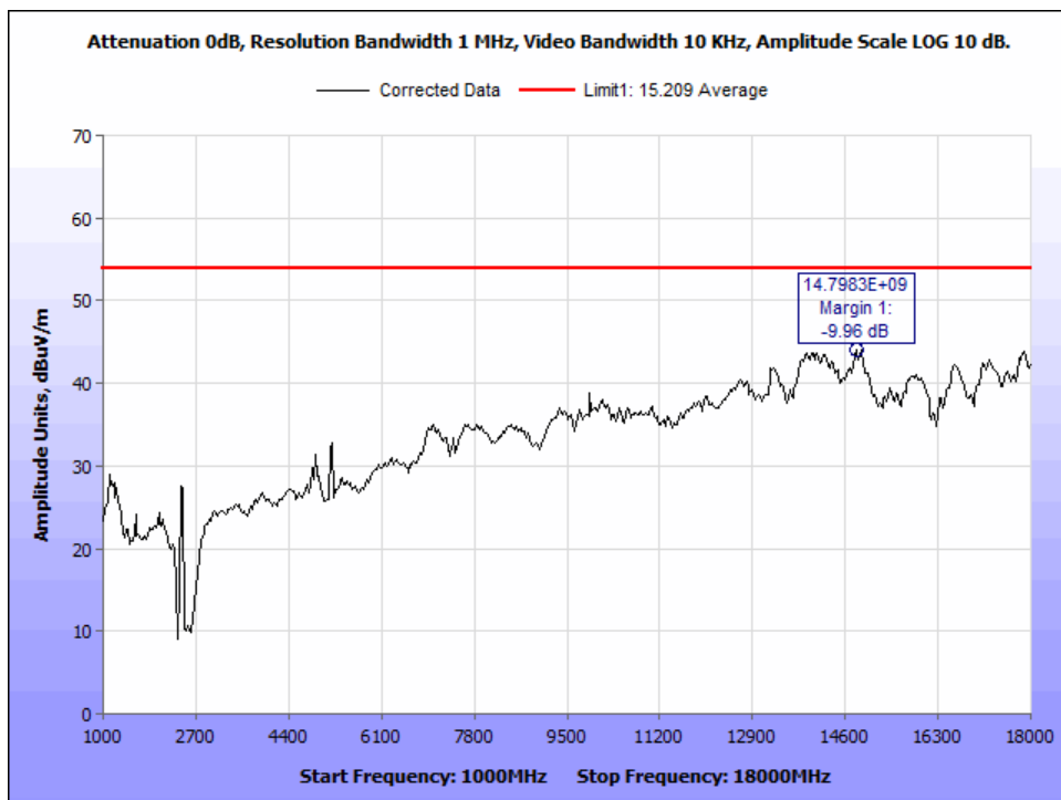
Figure 27: DH3_hopping_AVG Radiated Emissions_1-18 GHz.
