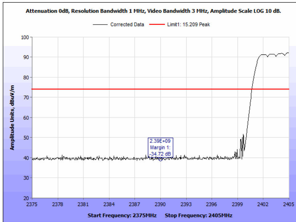
Figure 60: PK_DH3_Radiated Band Edge_2390MHz_hopping.
