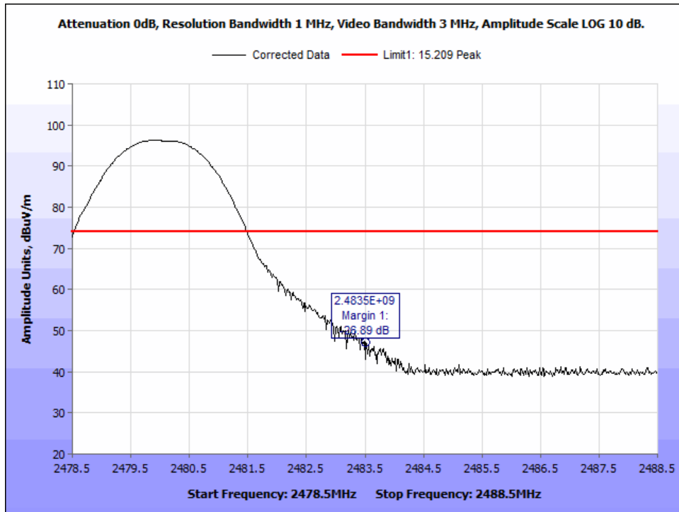
Figure 57: PK_DH1_Radiated Band Edge_2483.5MHz_CF 2480 MHz.
