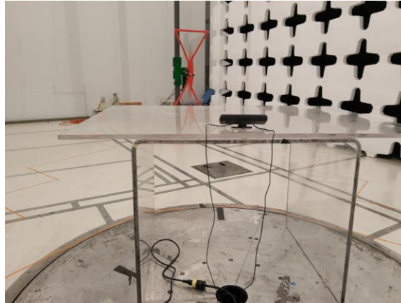
Figure 40: REE Test Setup - 30-1000MHz
