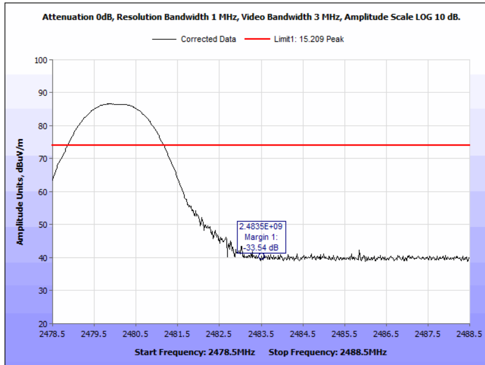
Figure 61: PK_DH3_Radiated Band Edge_2483.5MHz_CF 2480 MHz.
