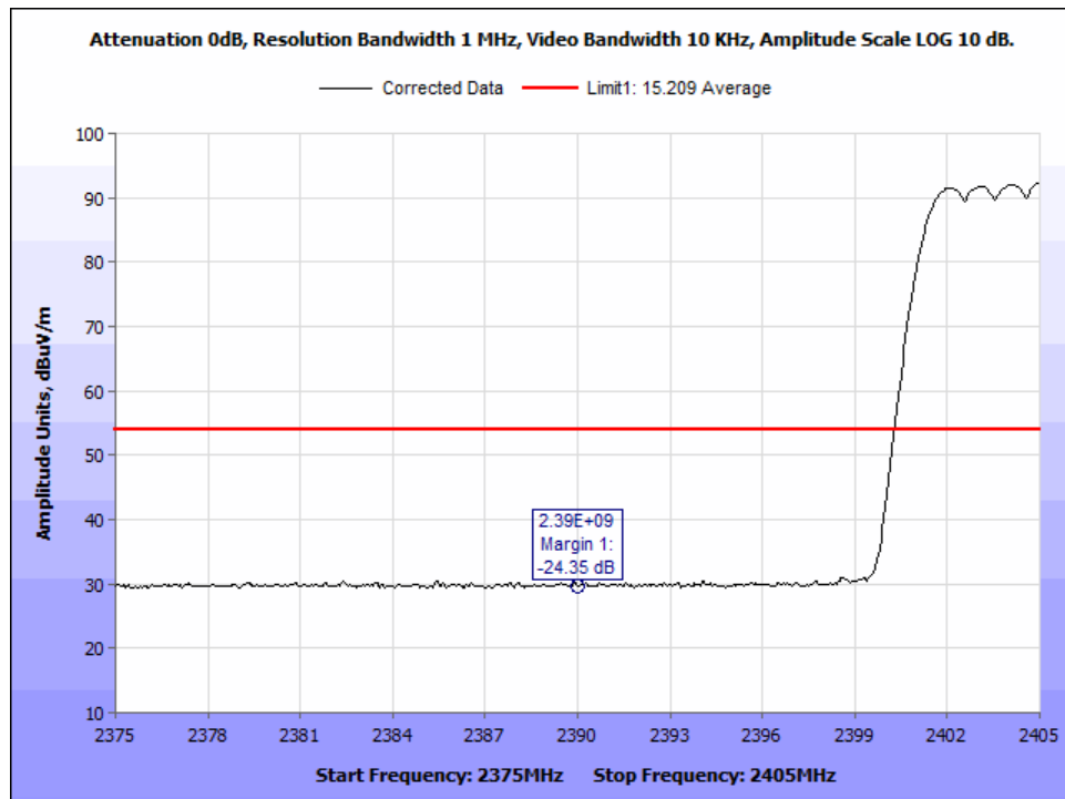
Figure 52: AVG_DH5_Radiated Band Edge_2390MHz_hopping.
