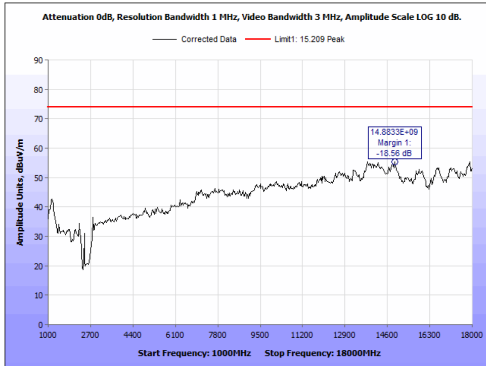
Figure 24: DH3_ch 2440_PK Radiated Emissions_1-18 GHz.
