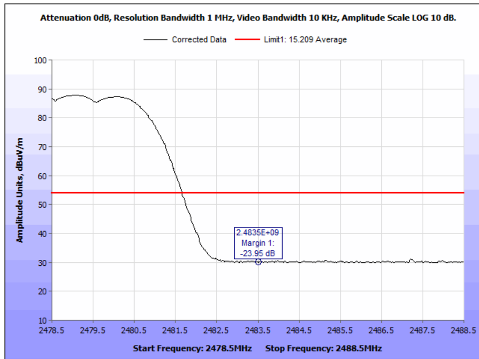
Figure 54: AVG_DH5_Radiated Band Edge_2483.5MHz_hopping.
