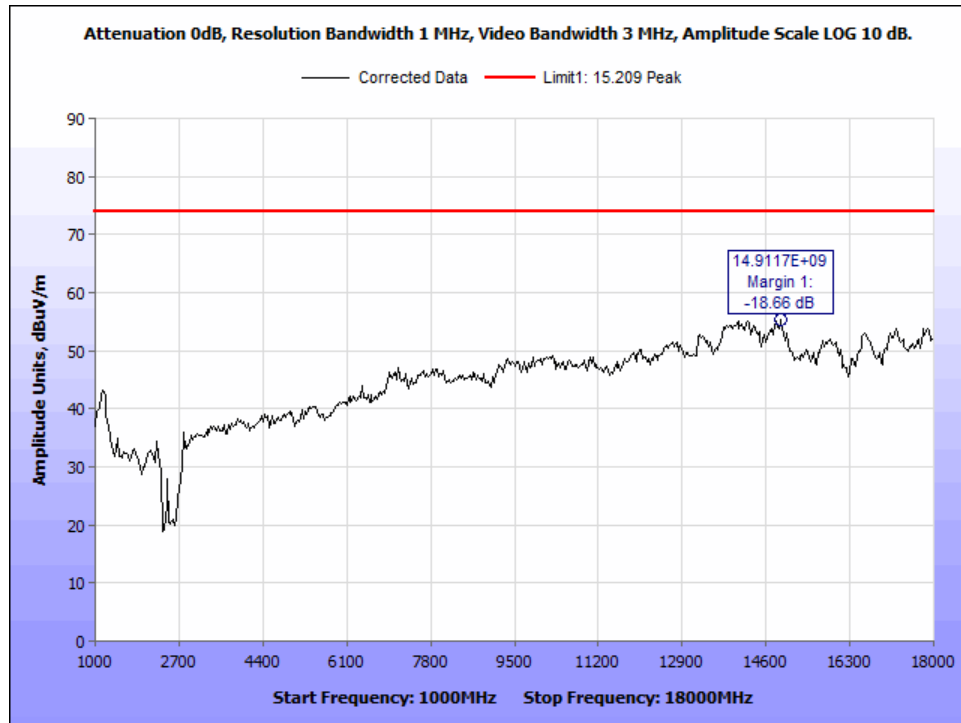
Figure 34: DH5_ch 2480_PK Radiated Emissions_1-18 GHz.
