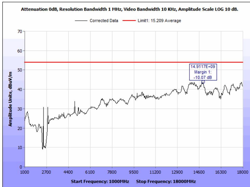
Figure 23: DH3_ch 2440_AVG Radiated Emissions_1-18 GHz.
