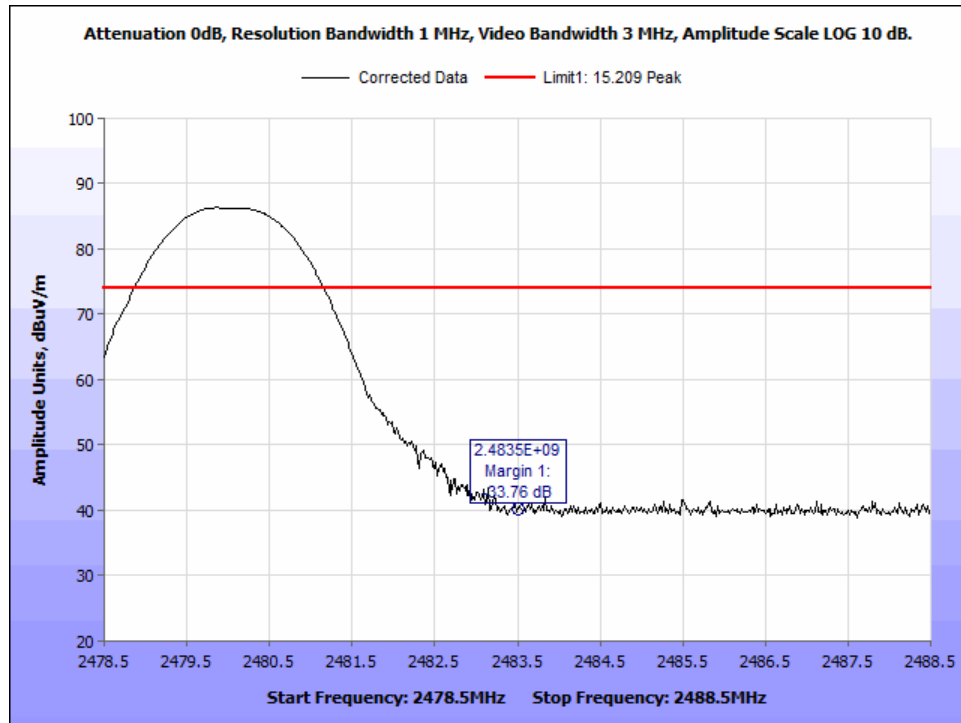
Figure 65: PK_DH5_Radiated Band Edge_2483.5MHz_CF 2480 MHz.
