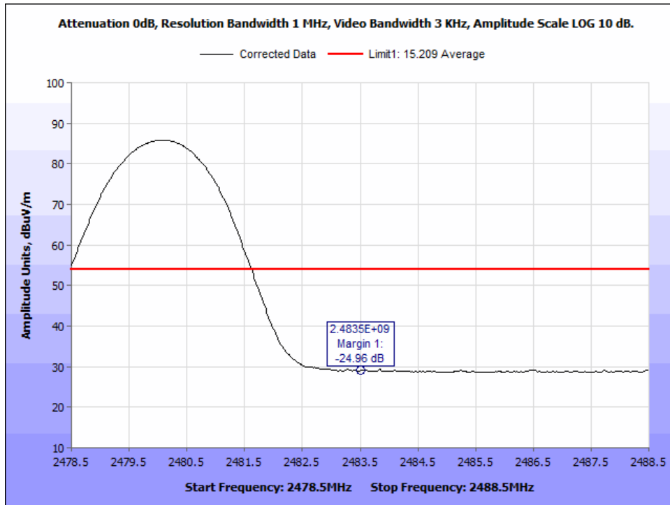
Figure 49: AVG_DH3_Radiated Band Edge_2483.5MHz_CF 2480 MHz.
