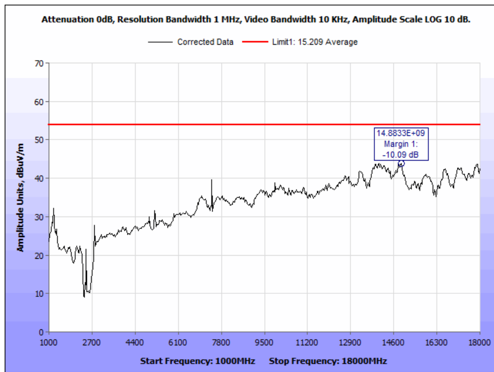
Figure 25: DH3_ch 2480_AVG Radiated Emissions_1-18 GHz.
