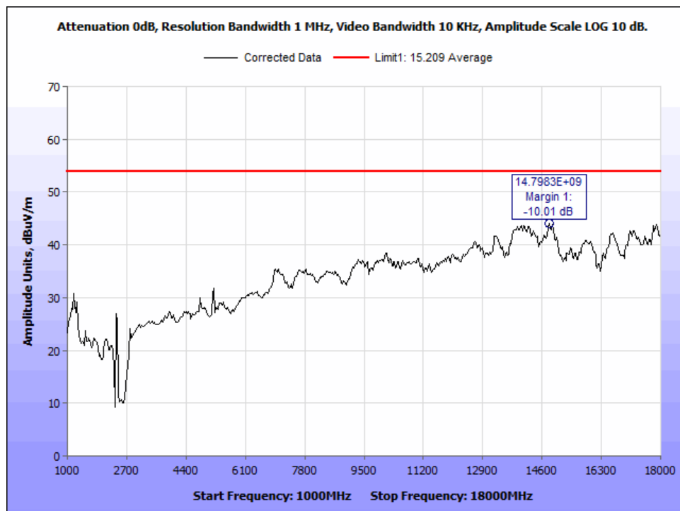
Figure 21: DH3_ch 2402_AVG Radiated Emissions_1-18 GHz.
