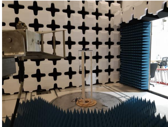
Figure 41: REE Test Setup - 1-18 GHz
