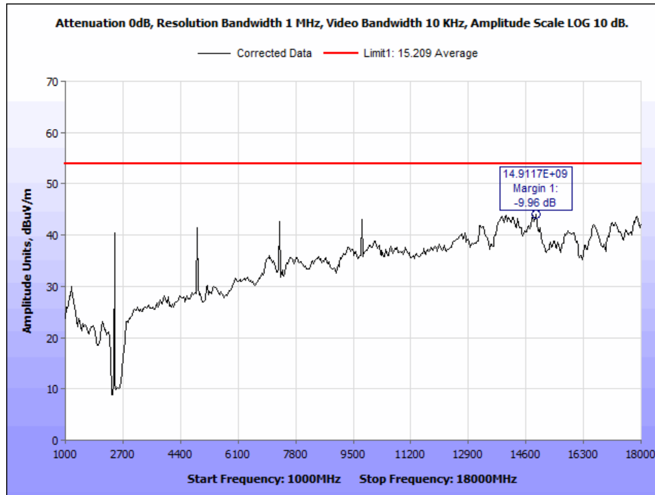
Figure 14: DH1_ch 2440_AVG Radiated Emissions_1-18 GHz.
