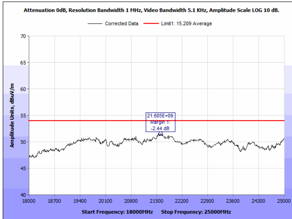
Figure 38: Average Radiated Emissions_worst case_18-25 GHz.
