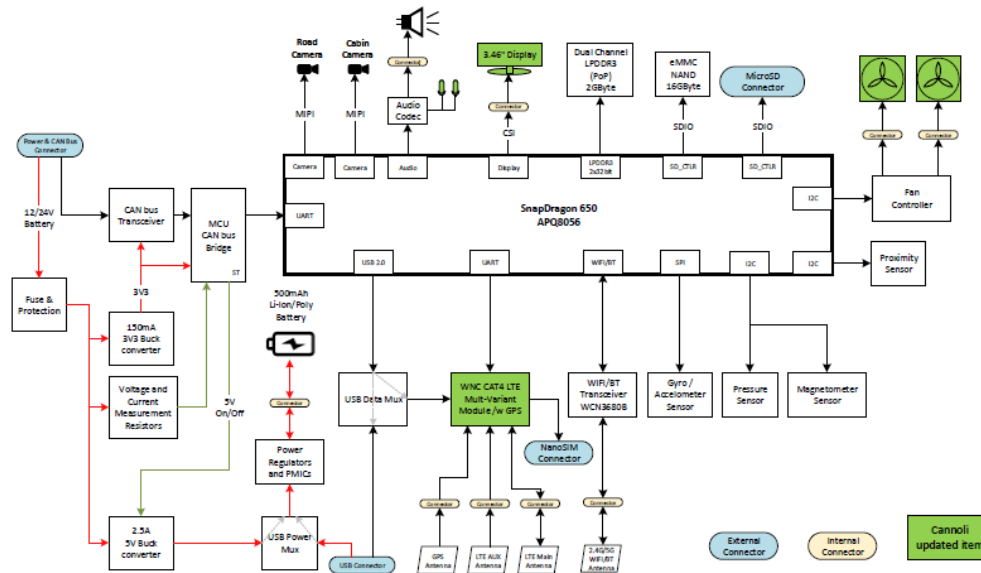
Figure 6: Block Diagram of Test Configuration
