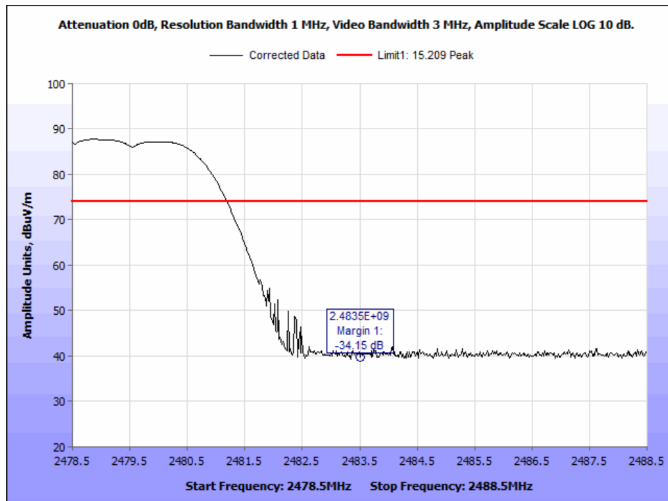
Figure 62: PK_DH3_Radiated Band Edge_2483.5MHz_hopping.
