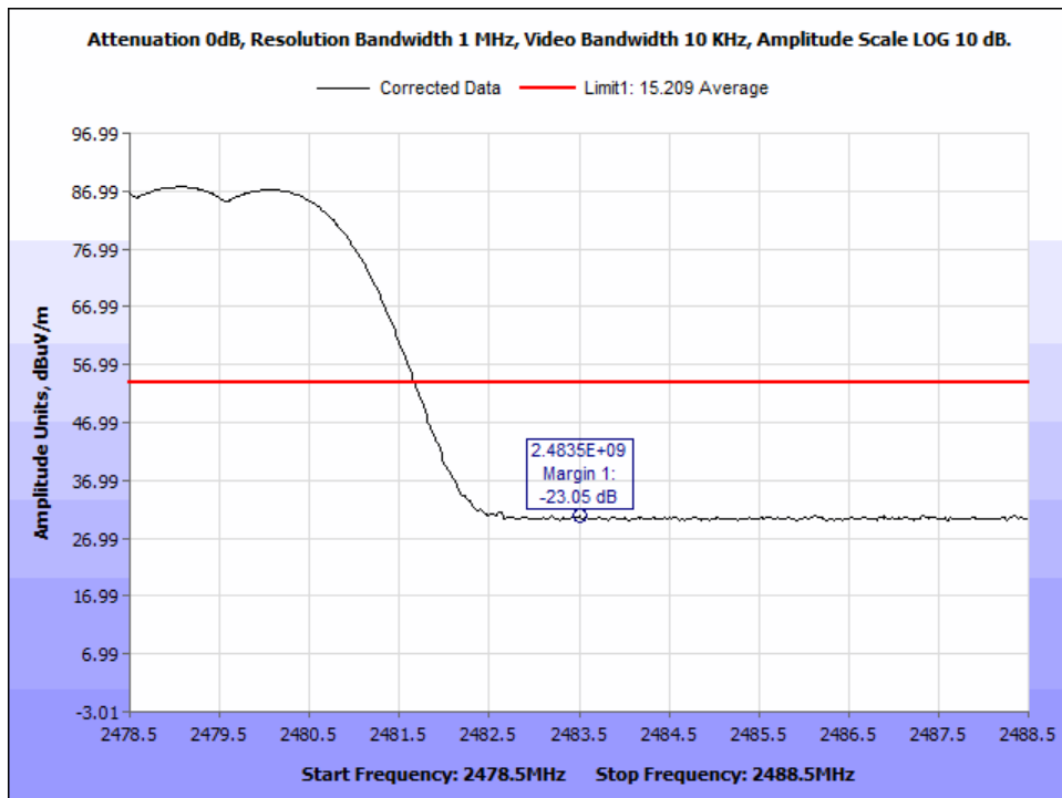
Figure 50: AVG_DH3_Radiated Band Edge_2483.5MHz_hopping.
