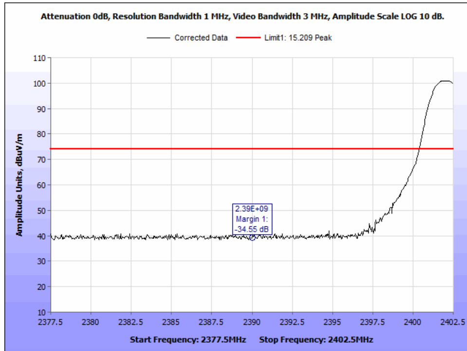
Figure 55: PK_DH1_Radiated Band Edge_2390MHz_CF 2402 MHz.
