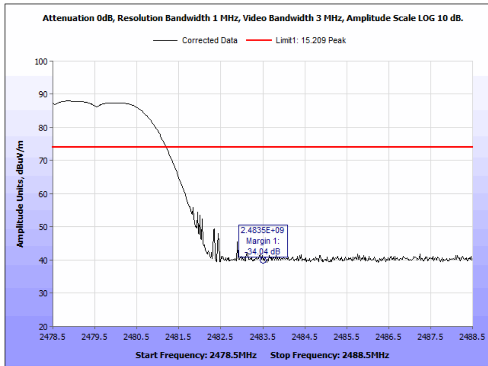
Figure 66: PK_DH5_Radiated Band Edge_2483.5MHz_hopping.
