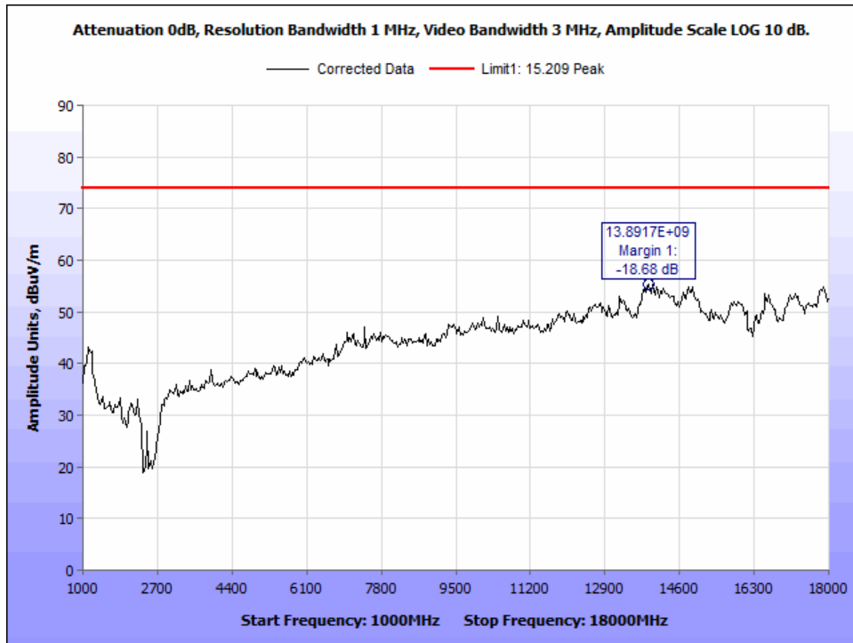
Figure 26: DH3_ch 2480_PK Radiated Emissions_1-18 GHz.
