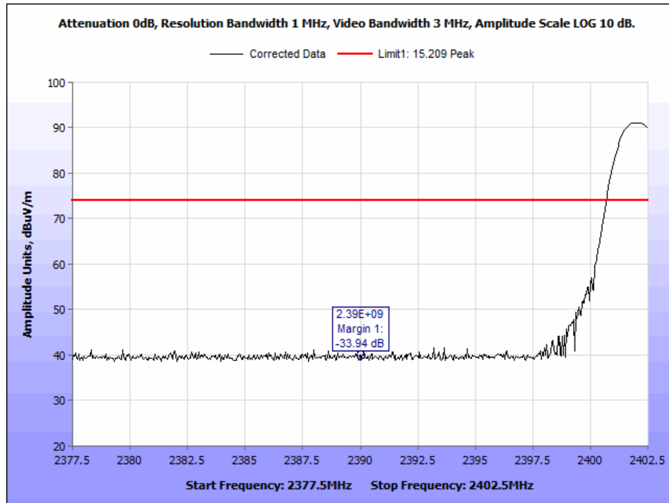
Figure 59: PK_DH3_Radiated Band Edge_2390MHz_CF 2402 MHz.
