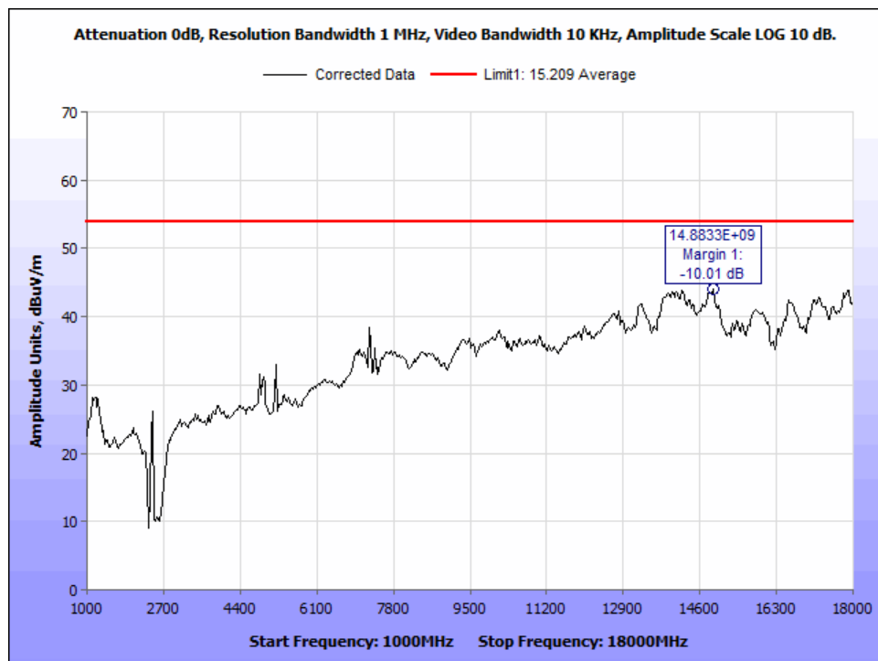
Figure 35: DH5_hopping_AVG Radiated Emissions_1-18 GHz.
