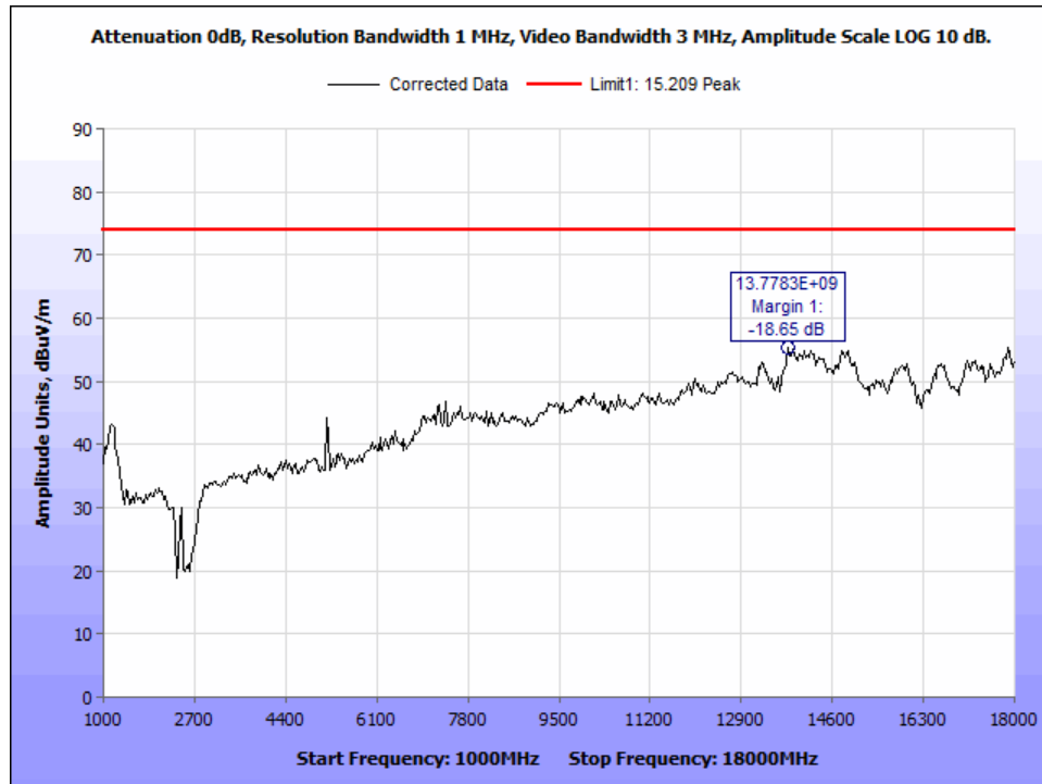
Figure 36: DH5_hopping_PK Radiated Emissions_1-18 GHz.
