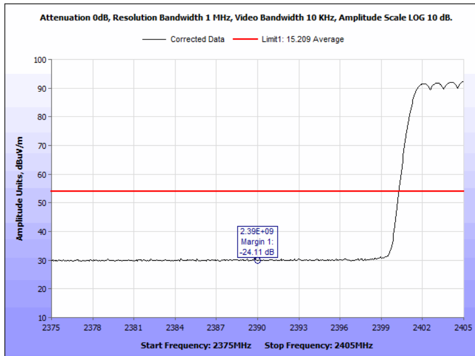
Figure 48: AVG_DH3_Radiated Band Edge_2390MHz_hopping.
