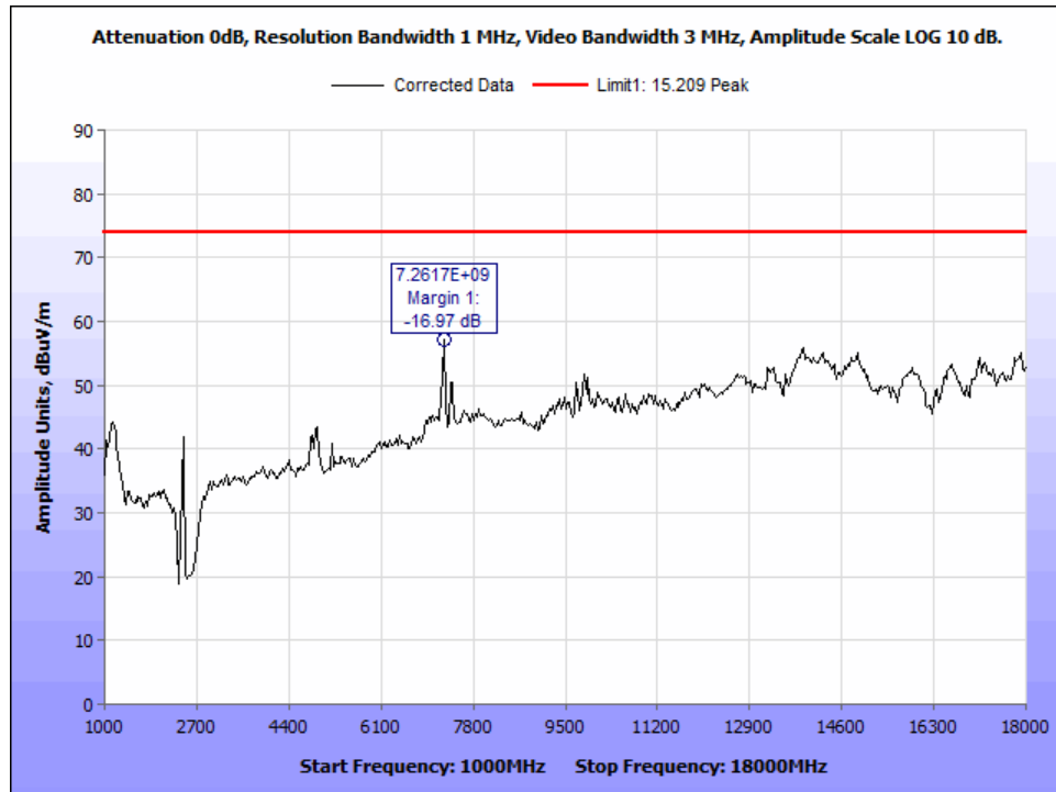
Figure 20: DH1_hopping_PK Radiated Emissions_1-18 GHz.
