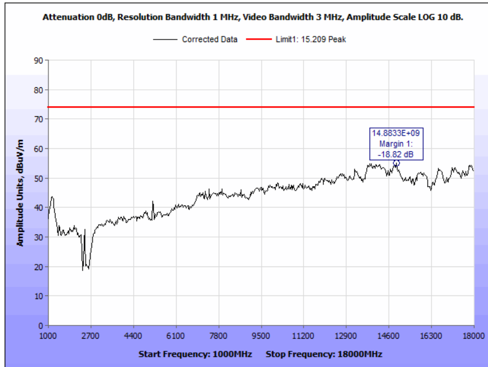
Figure 28: DH3_hopping_PK Radiated Emissions_1-18 GHz.
