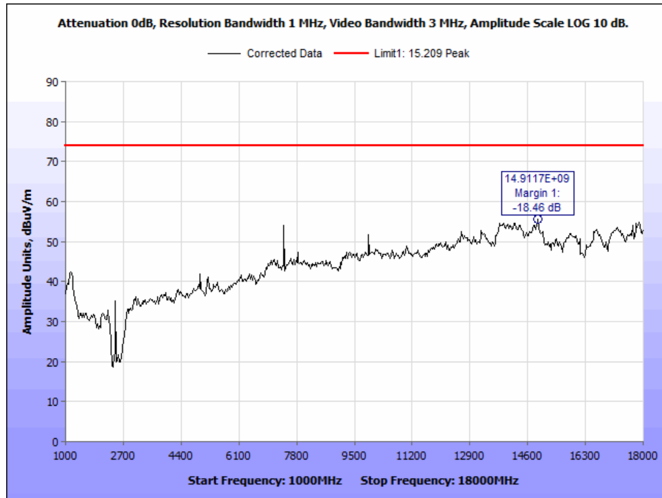
Figure 18: DH1_ch 2480_PK Radiated Emissions_1-18 GHz.
