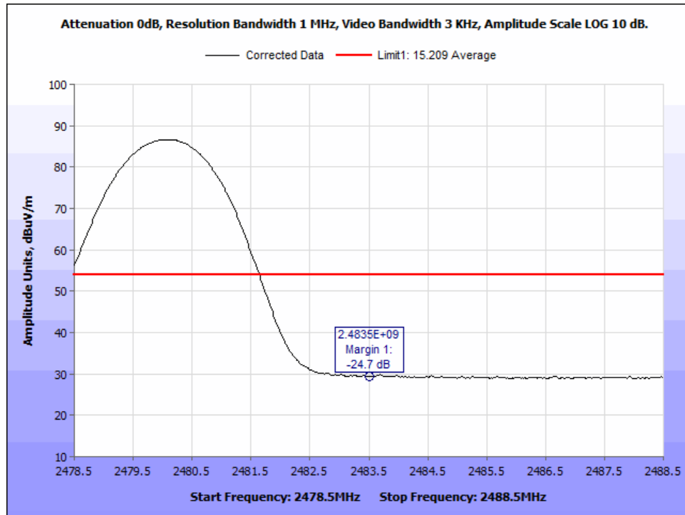
Figure 53: AVG_DH5_Radiated Band Edge_2483.5MHz_CF 2480 MHz.
