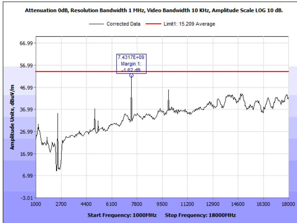
Figure 16: DH1_ch 2480_AVG Radiated Emissions_1-18 GHz.
