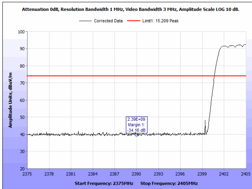
Figure 64: PK_DH5_Radiated Band Edge_2390MHz_hopping.
