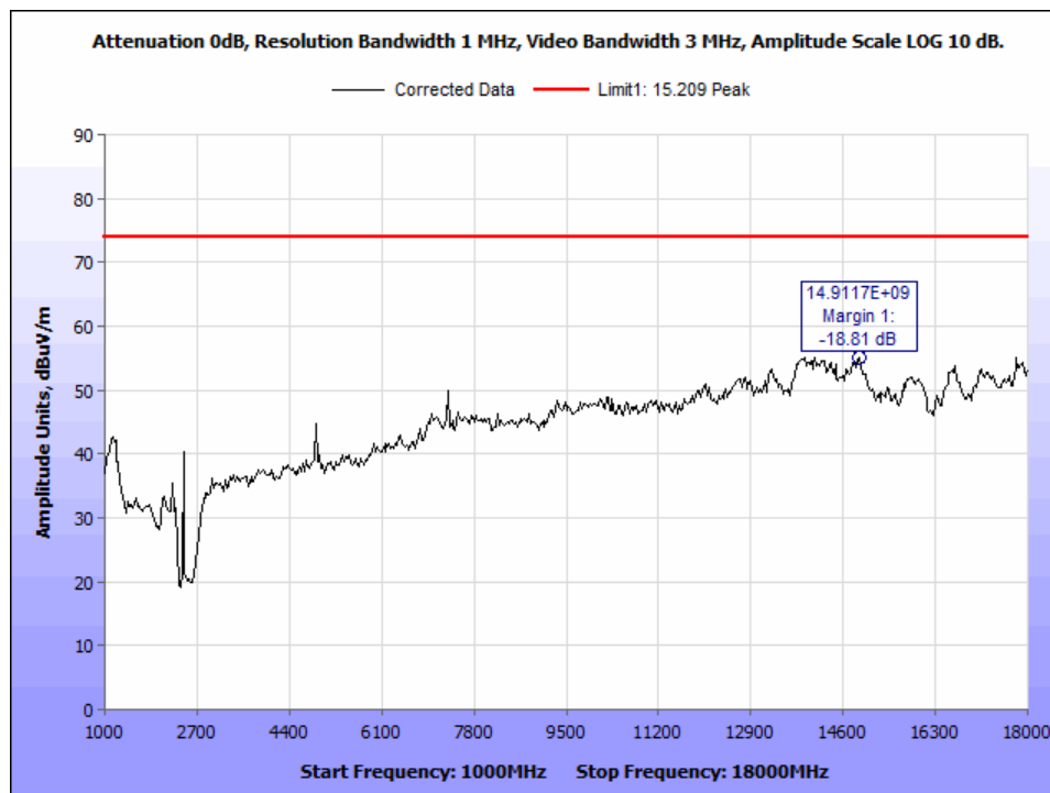
Figure 15: DH1_ch 2440_PK Radiated Emissions_1-18 GHz.
