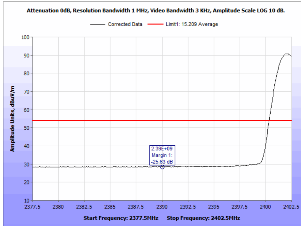
Figure 51: AVG_DH5_Radiated Band Edge_2390MHz_CF 2402 MHz.
