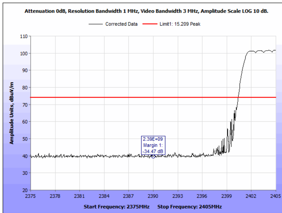
Figure 56: PK_DH1_Radiated Band Edge_2390MHz_hopping.
