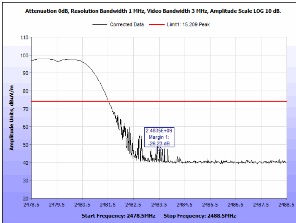
Figure 58: PK_DH1_Radiated Band Edge_2483.5MHz_hopping.
