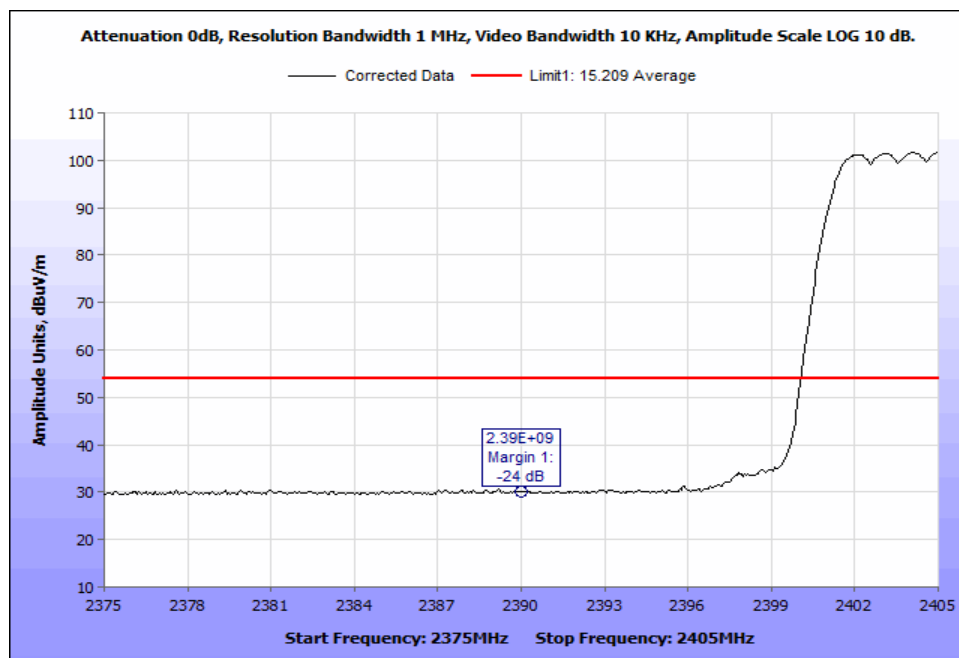
Figure 44: AVG_DH1_Radiated Band Edge_2390MHz_hopping.
