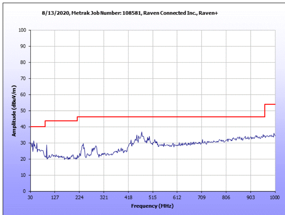
Figure 37: worst case_Radiated Emissions_30-1000MHz.
