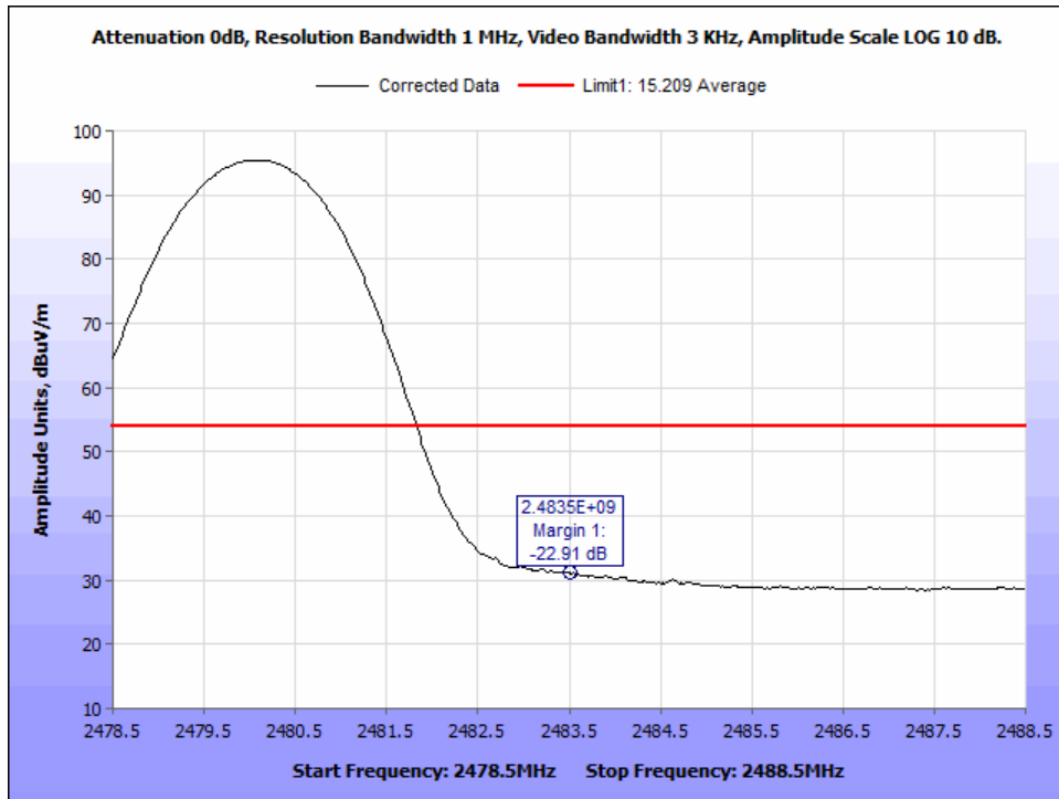
Figure 45: AVG_DH1_Radiated Band Edge_2483.5MHz_CF 2480 MHz.
