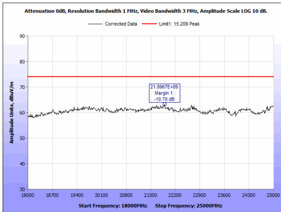
Figure 39: Peak Radiated Emissions_worst case_18-25 GHz.
