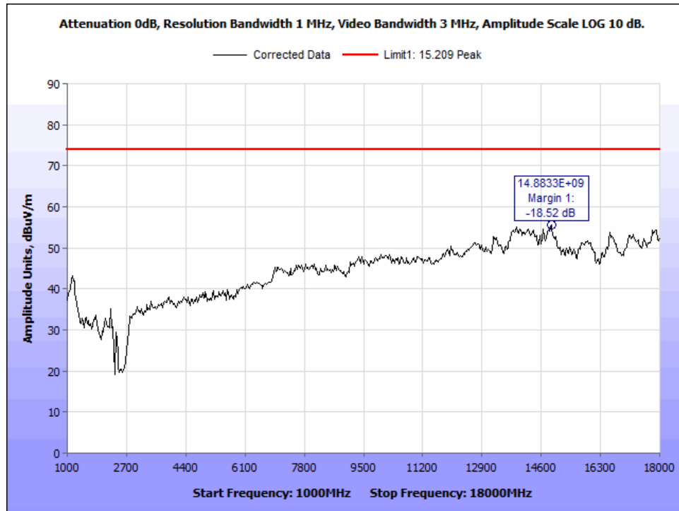
Figure 30: DH5_ch 2402_PK Radiated Emissions_1-18 GHz.
