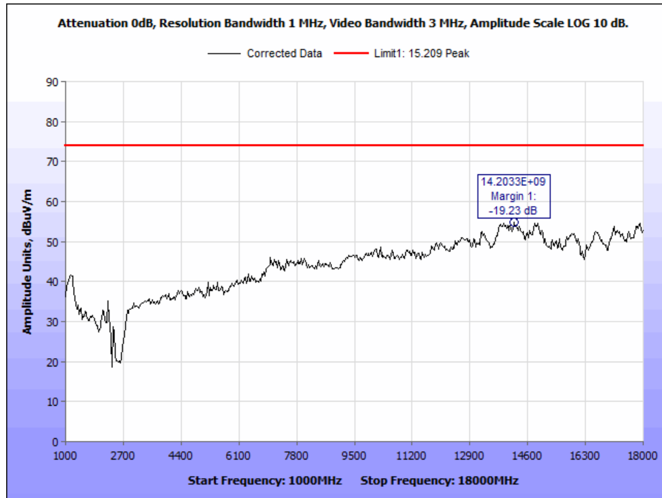
Figure 22: DH3_ch 2402_PK Radiated Emissions_1-18 GHz.
