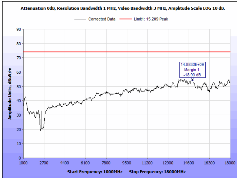
Figure 32: DH5_ch 2440_PK Radiated Emissions_1-18 GHz.
