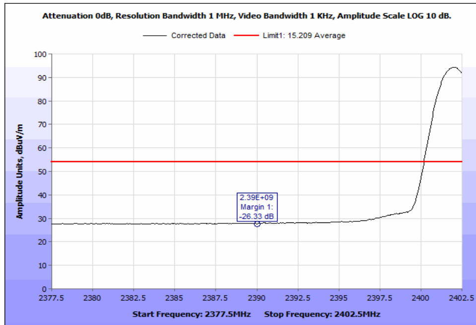
Figure 43: AVG_DH1_Radiated Band Edge_2390MHz_CF 2402 MHz.
