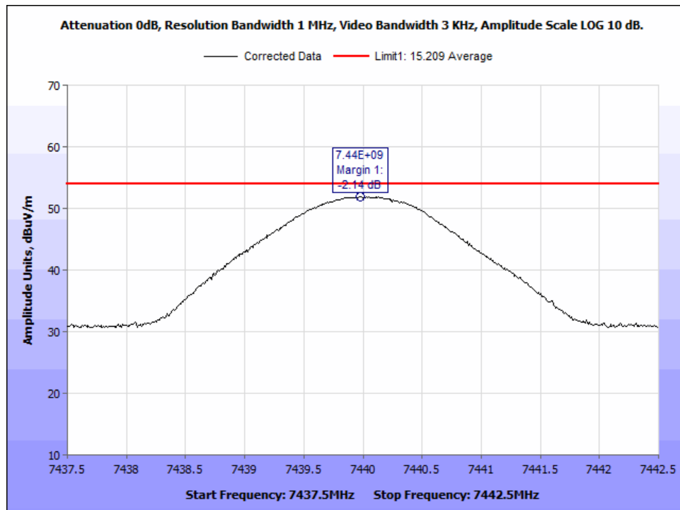
Figure 17: DH1_ch 2480_AVG Radiated Emissions_3x harmonic.
