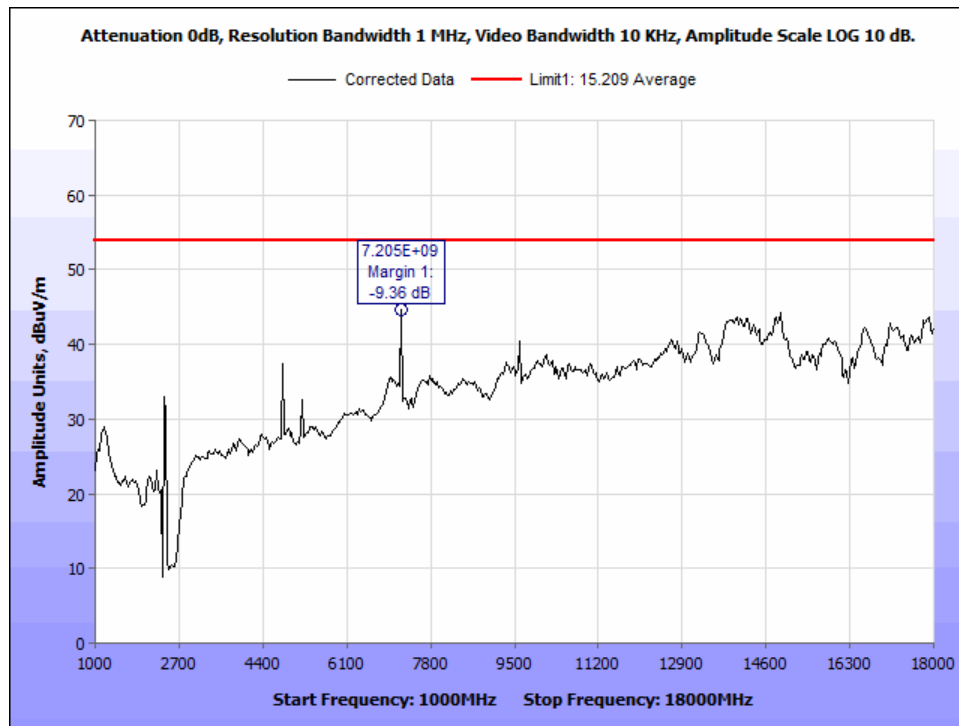
Figure 12: DH1_ch 2402_AVG Radiated Emissions_1-18 GHz.
