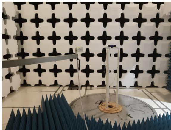
Figure 42: REE Test Setup - 18-40 GHz
