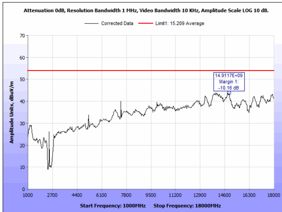
Figure 33: DH5_ch 2480_AVG Radiated Emissions_1-18 GHz.
