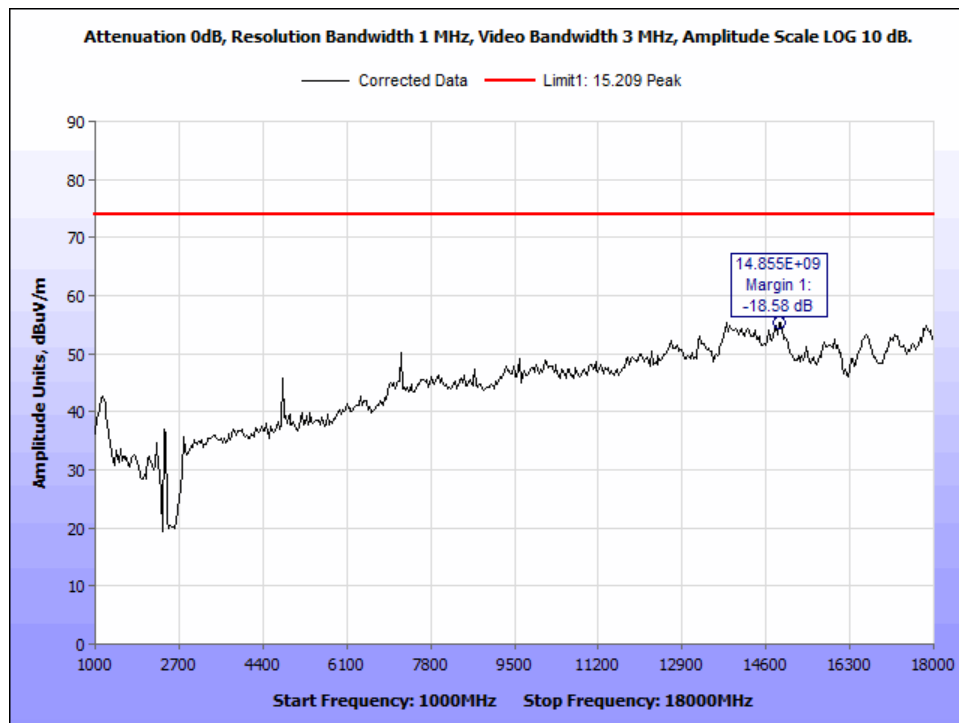
Figure 13: DH1_ch 2402_PK Radiated Emissions_1-18 GHz.
