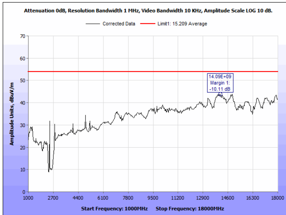
Figure 31: DH5_ch 2440_AVG Radiated Emissions_1-18 GHz.
