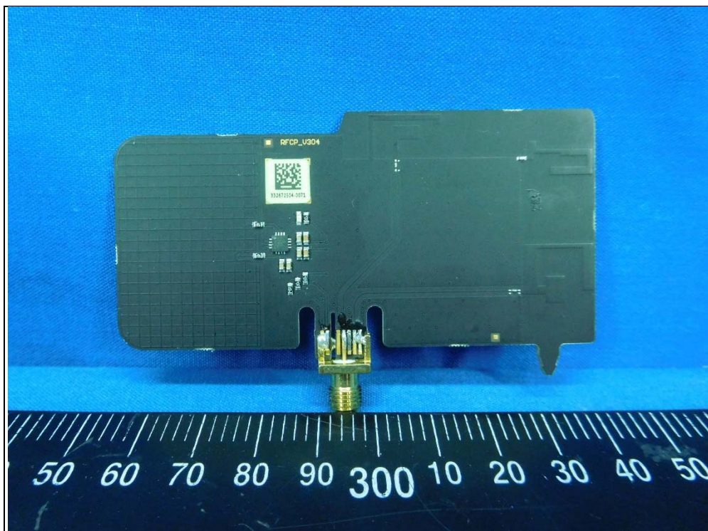
Antenna set 5 (Model: DVT-BA-M-1311-P)
