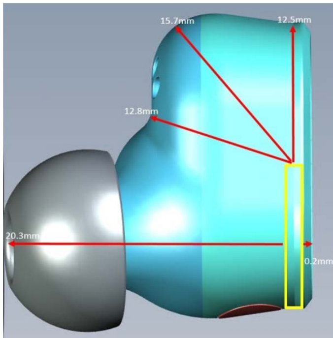
Left Earbud
