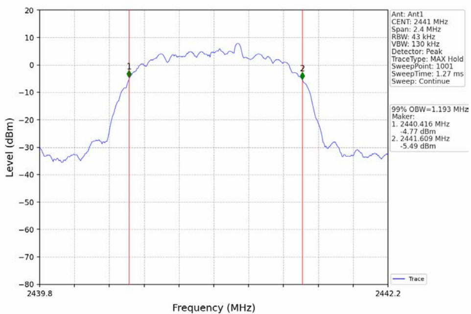
8DPSK_3DH5_MCH_2441MHz_Ant1_NTNV
