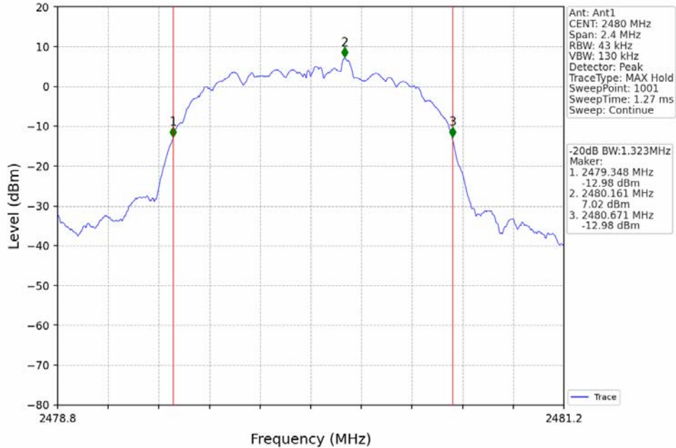
8DPSK_3DH5_HCH_2480MHz_Ant1_NTNV
