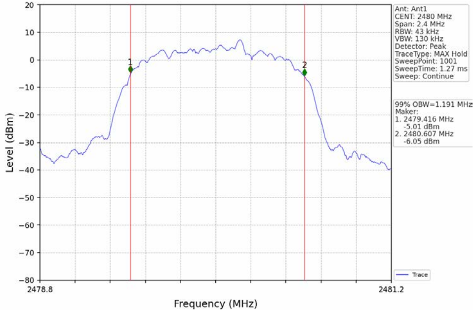
8DPSK_3DH5_HCH_2480MHz_Ant1_NTNV
