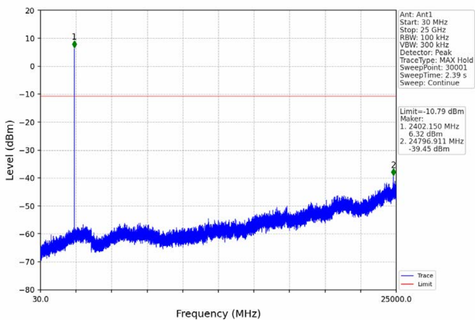
8DPSK_3DH5_LCH_2402MHz_Ant1_NTNV
