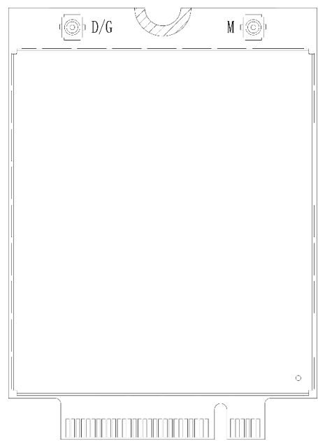
Figure 16. RF connectors
