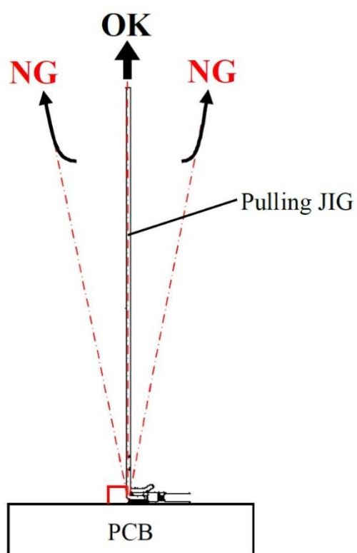
Figure 23. Pulling direction
