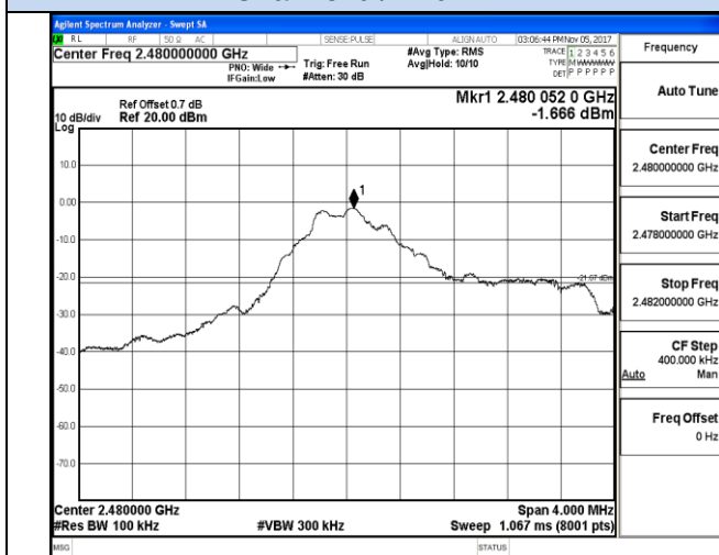
Channel 18 / 2480 MHz
