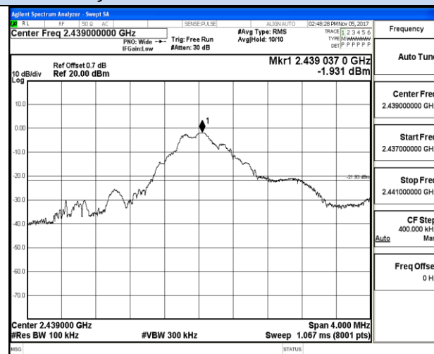
Channel 09 / 2439 MHz
