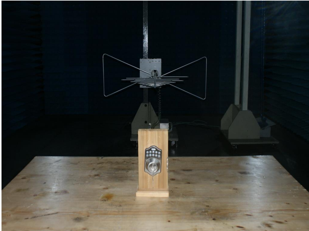
Photograph 3: Set-up for Spurious Emissions (30MHz-1GHz)
