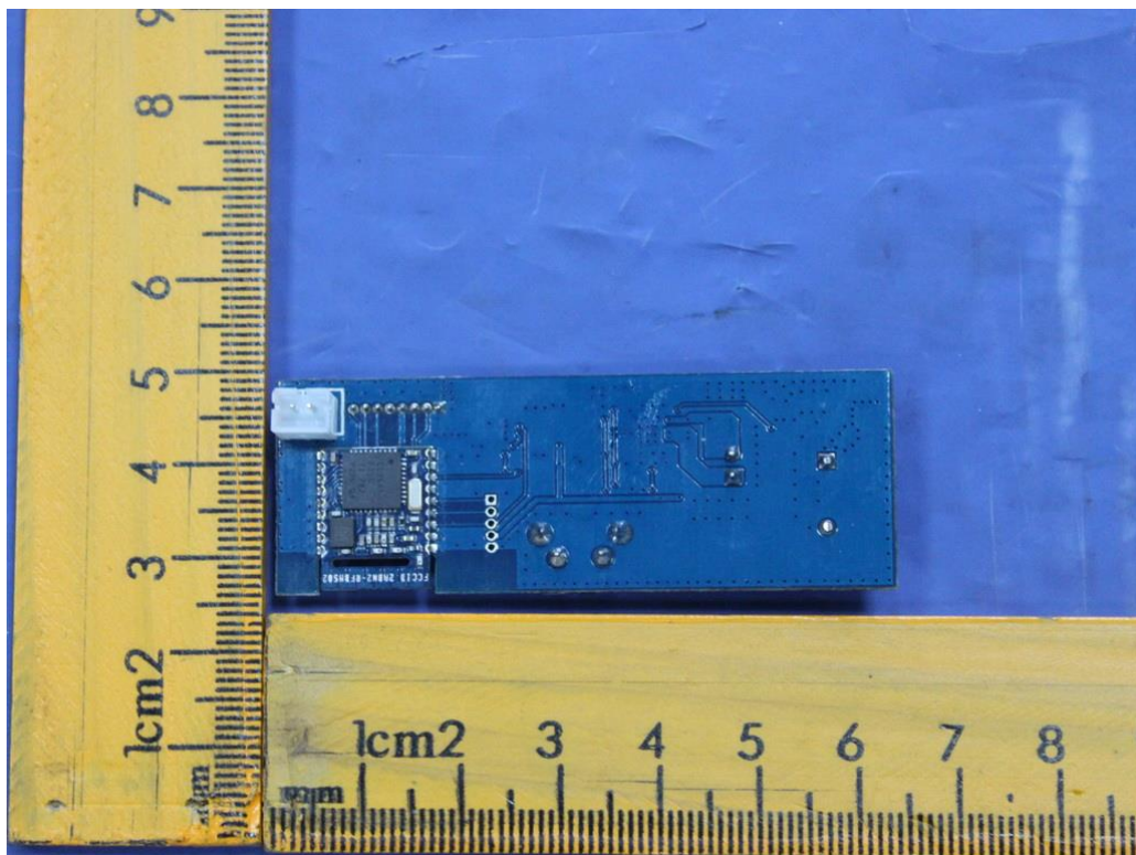
Fig. 8: Internal view
