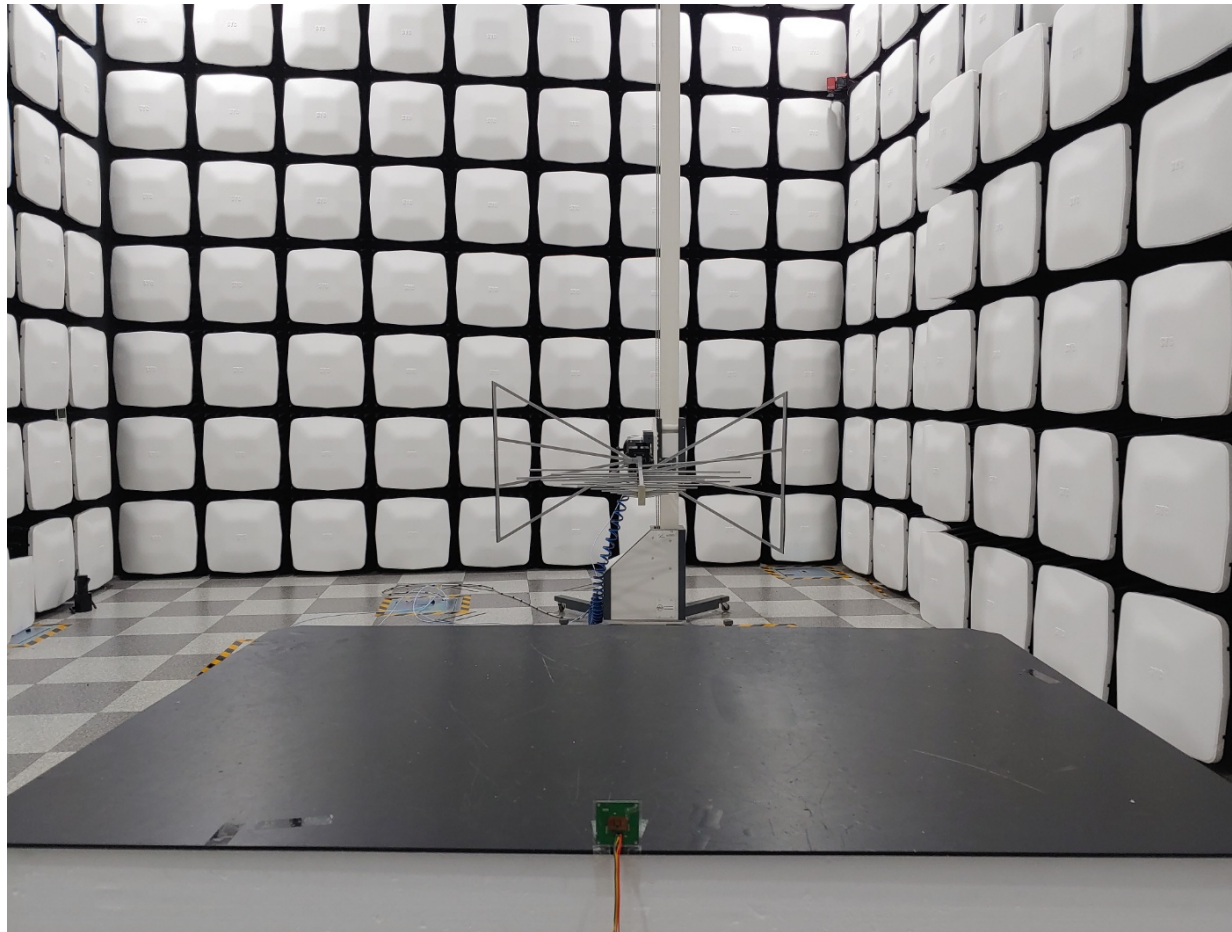
Radiated RF measurement (Below 1 GHz)
