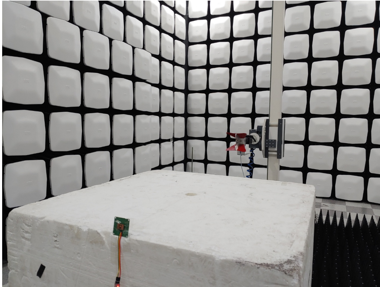
Radiated RF measurement (Above 1 GHz)
